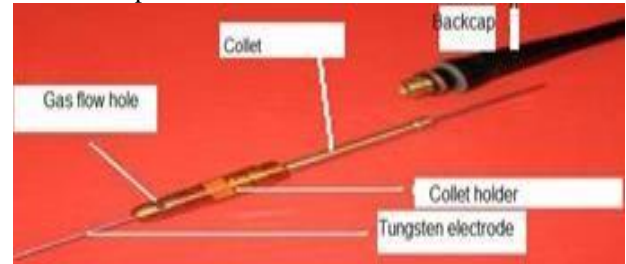
TIG torch components
