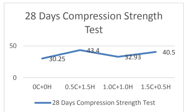
Graph 2 Compressive strength of M40 Grade mix with various % of fibers at the age of 7 & 28 days.
