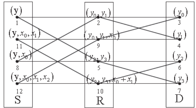
Fig. 3. Implementation of the successive cancellation decoder.
