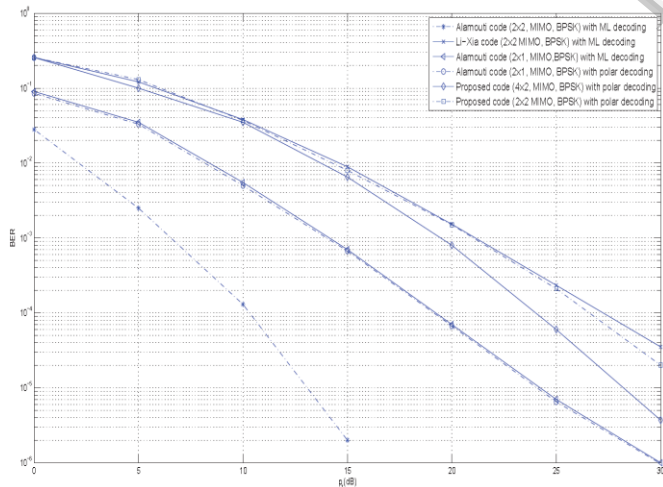
Fig. 4. BER performance behaviors with polar decoding.
