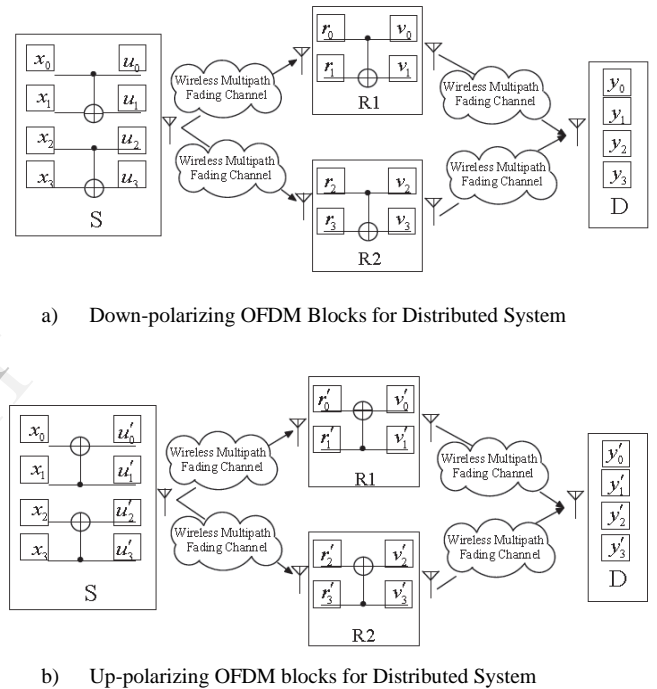
Fig. 1. The relay communication system based on the polarizing MIMO-OFDM channels with two models: (a) denotes the down-polarizing communication model; and (b) denotes the up-polarizing communication model.
