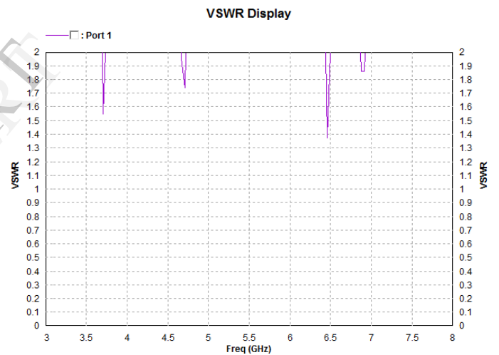
Figure 7: VSWR
