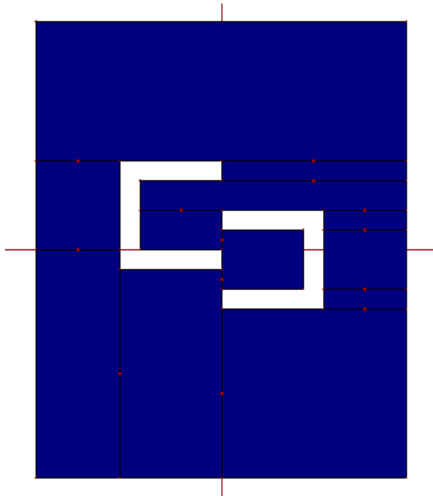
Figure 1: C slots etched on Rectangular Patch Antenna
