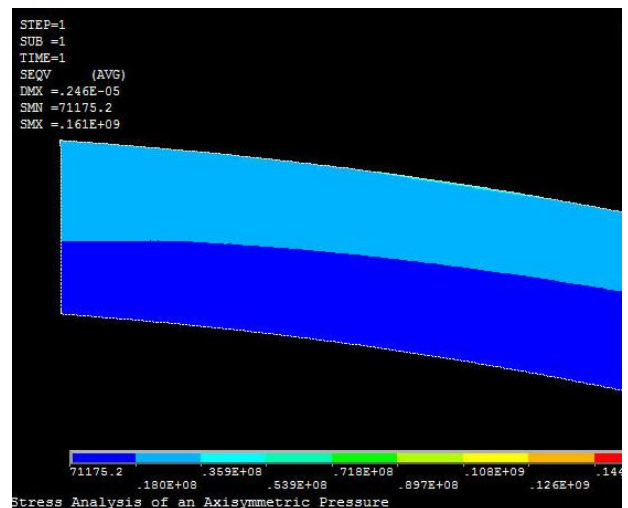
Von MISES stress at crown of head of the existing model
