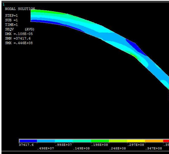
VON MISES stress at crown of head of the new model
