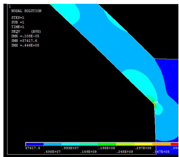
VON MISES stress at equator of the head of new model
