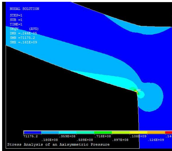
VON MISES stress at equator of head of the existing model
