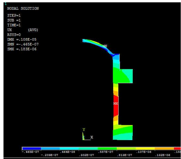
Nodal displacement in new model
