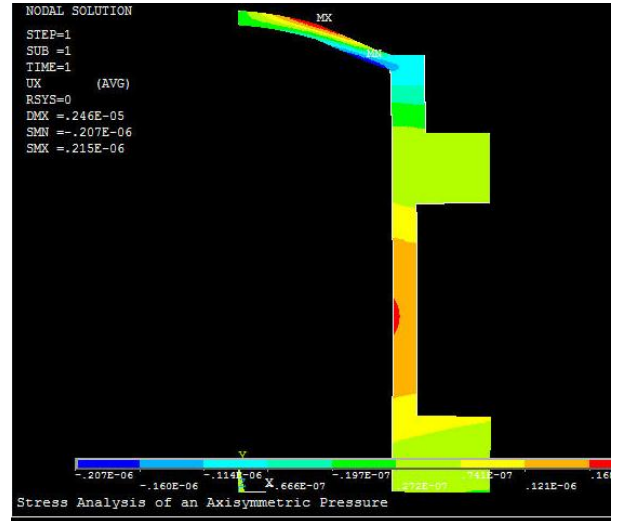
Nodal displacement in existing model
