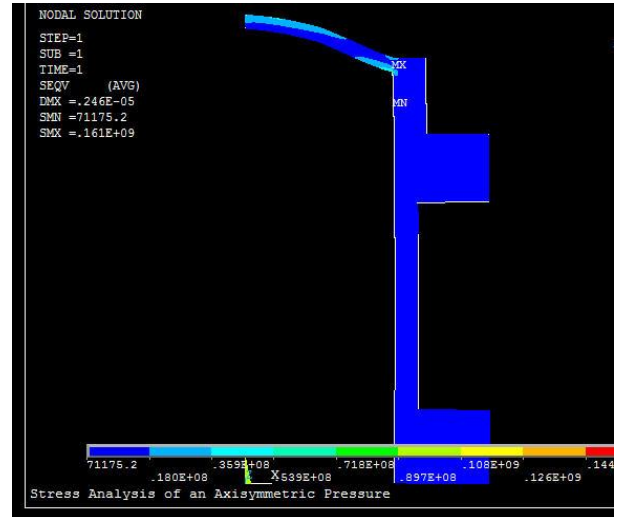
Von Mises Stress of existing model
