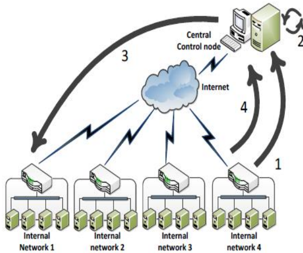
Fig. 3 The workflow of Garlic.
