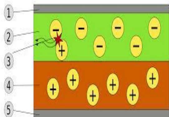
Fig. 2: Bilayer Oled: 1. Cathode (-), 2. Emissive Layer, 3. Emission Of Radiation, 4. Conductive Layer, 5. Anode (+)
