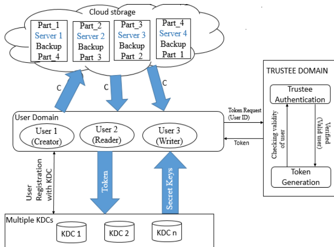
Fig.1.A Secured Proposed Architecture
