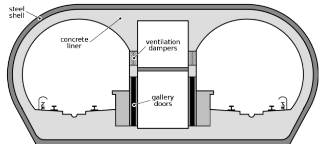
Fig-4:Crosssectionoftransbaytube
