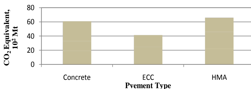
FIGURE 1 Greenhouse gas emissions during life-cycle (19)
