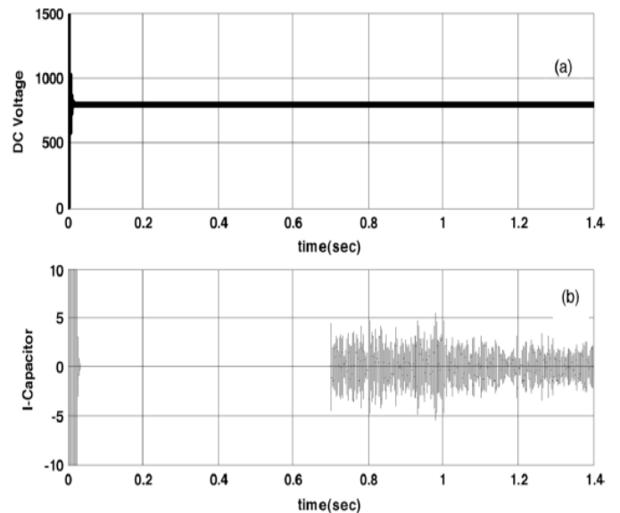
Fig. 7. (a) DC link voltage. (b) Current through Capacitor.
