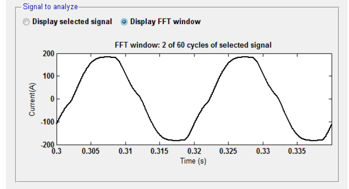
Fig. 10. (a) Source Current. (BALANCED LOAD)
