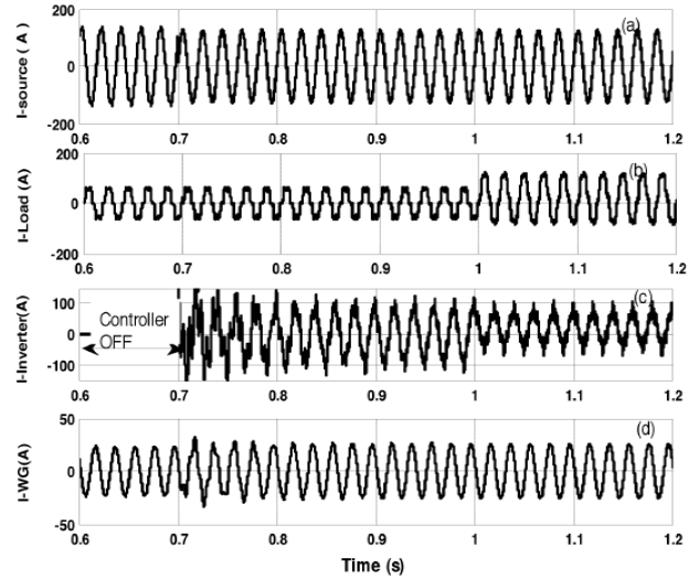
Fig. 6. (a) Source Current. (b) Load Current. (c) Inverter Injected Current. (d) Wind generator (Induction generator) current.
