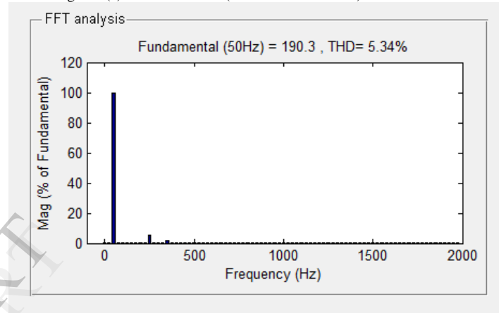
Fig. 10. (b) FFT of source current.
