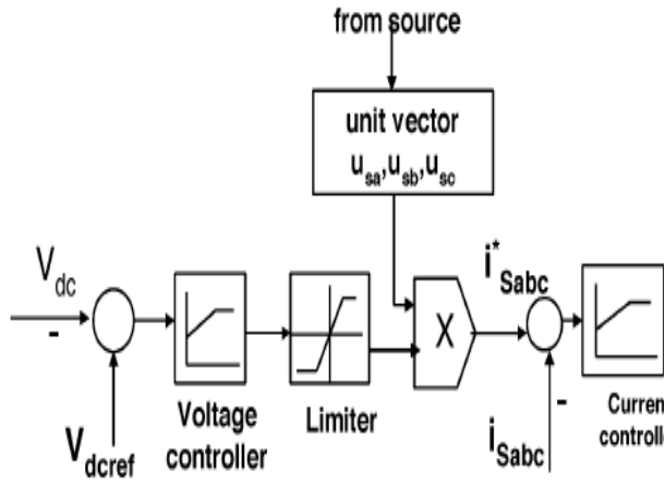
Fig. 3. Control system scheme.
