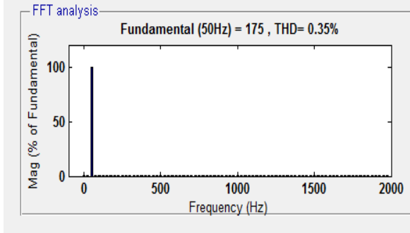
Fig. 11 (b) FFT of source current.
