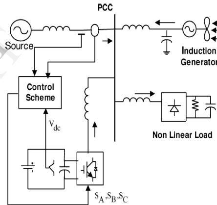
Fig. 2. System operational scheme in grid system.
