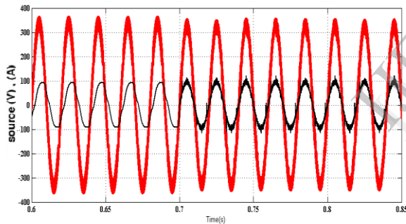
Fig. 9. Supply Voltage and Current at PCC.
