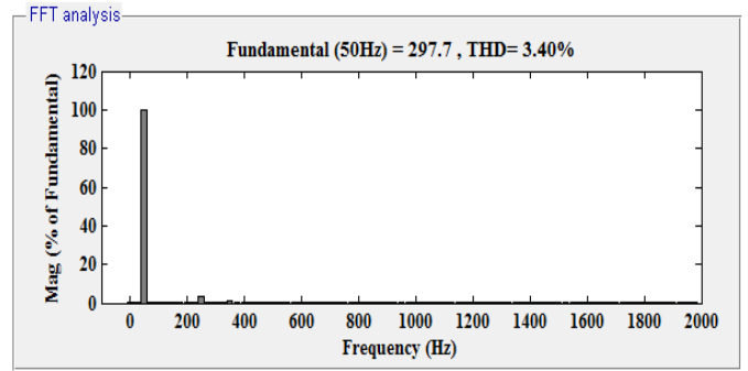
Fig. 12 (b) FFT of source current.
