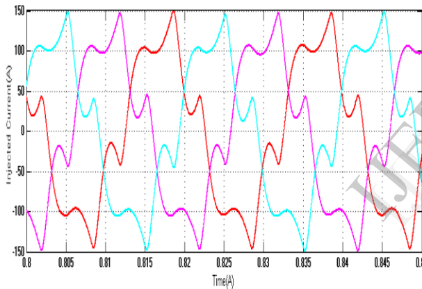
Fig.5.Threephase injected inverter Current.
