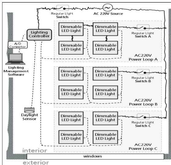
Fig. 5 Integration of the proposed lighting control system
