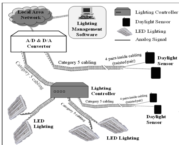
Fig. 1 Architecture design of the lighting system
