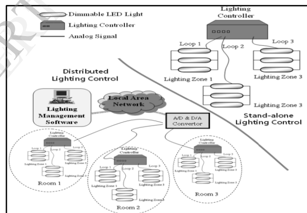
Fig. 4 Topology of the lighting control system
