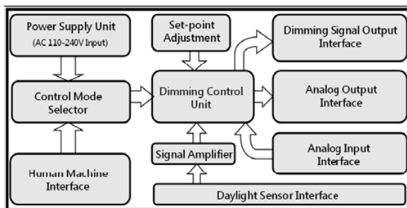
Fig. 3 Block diagram of the lighting controller design
