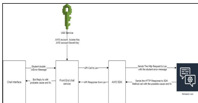
Fig. 1. Block diagram of C-Genie Model
