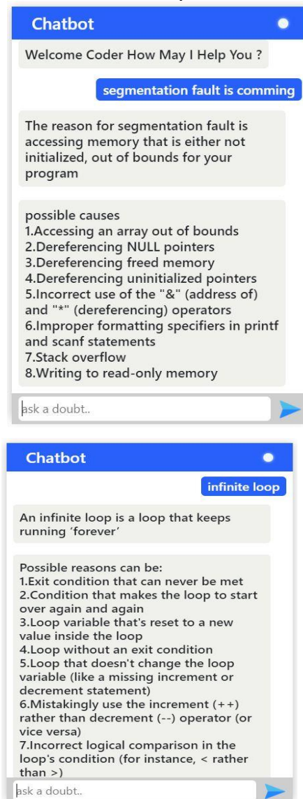
Fig. 2. Responses for segmentation fault error and infinite loop error
