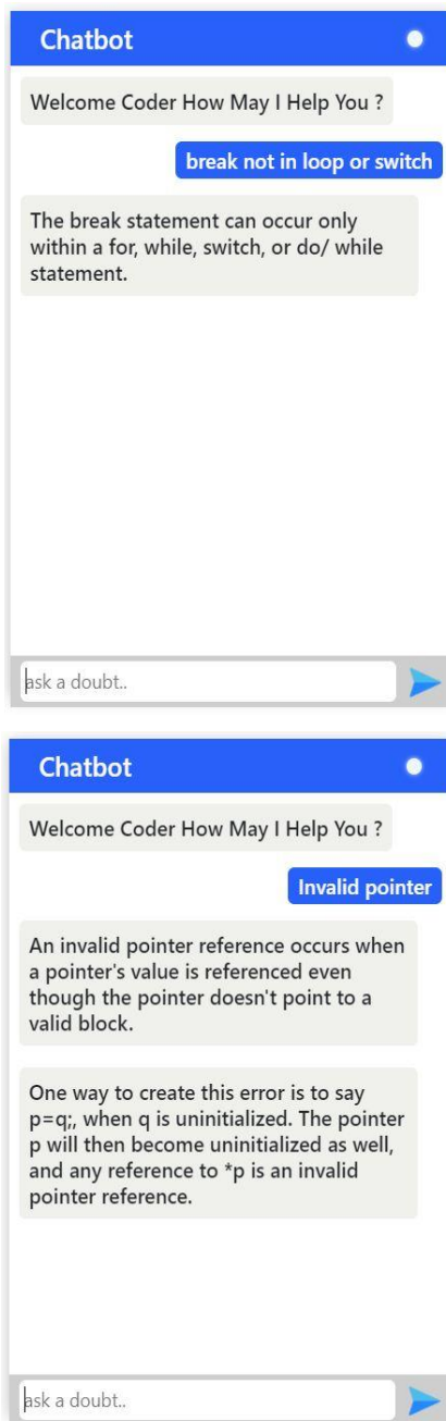
Fig. 3. C-Genie responses for common C errors
