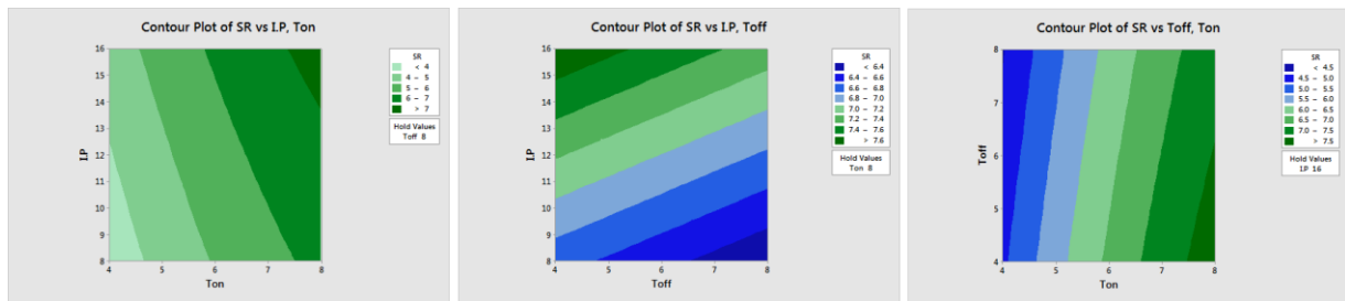
Fig. 6: Contour plots of SR showing the combined effects of pulse on time ( T_{on} ), Peak Current (LP) and Pulse off time ( T_{off} ) at higher value setting of constant parameter
