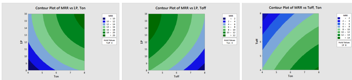
Fig. 1: Contour plots of MRR showing the combined effects of pulse on time (T on ), Peak Current (I.P) and Pulse off time (T off ) at lower value settings of constant parameter
