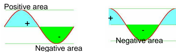
Fig 2.3.1 the area under a sine and a cosine wave over one period is always zero.
