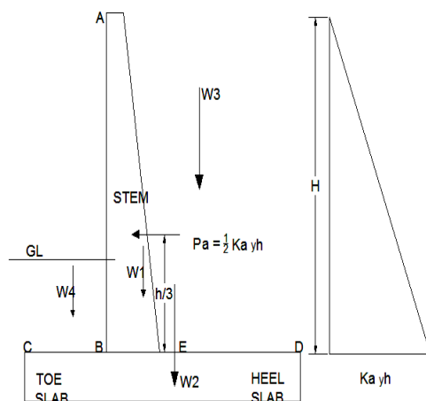
Fig.3: Mechanism of Cantilever Retaining Wall
