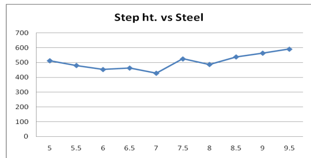
Graph 8: Step location Vs steel kg/m for wall Ht. 10.0 m
