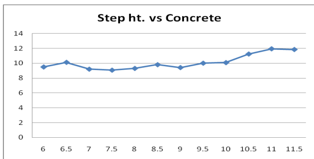
Graph 10: Step location Vs concrete cum/m for wall Ht. 12m
