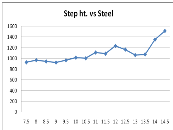
Graph 14: Step location Vs steel kg/m for wall Ht. 15.0m
