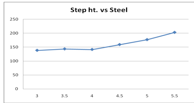
Graph 2: Step location Vs steel kg for wall Ht. 6.0 m
