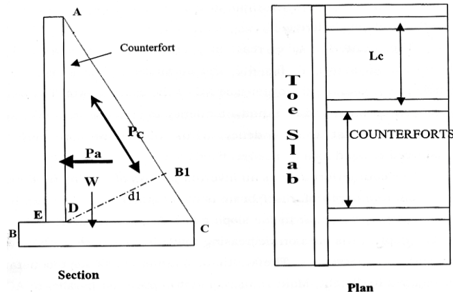
Fig.4: Mechanism of Counter fort Retaining Wall
