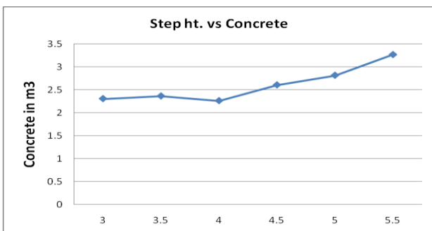
Graph 1: Step location Vs concrete m3 for wall Ht. 6.0 m
