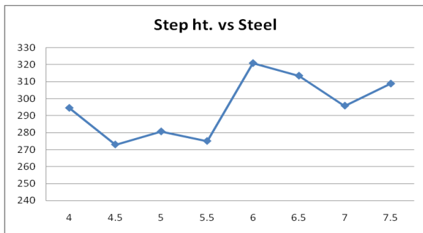
Graph 5: Step location Vs steel kg/m for wall Ht. 8m
