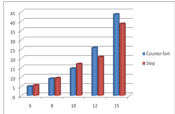
Graph 16: Concrete Quantity Comparison
