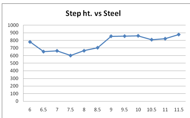
Graph 11: Step location Vs steel kg/m for wall Ht. 12.0 m
