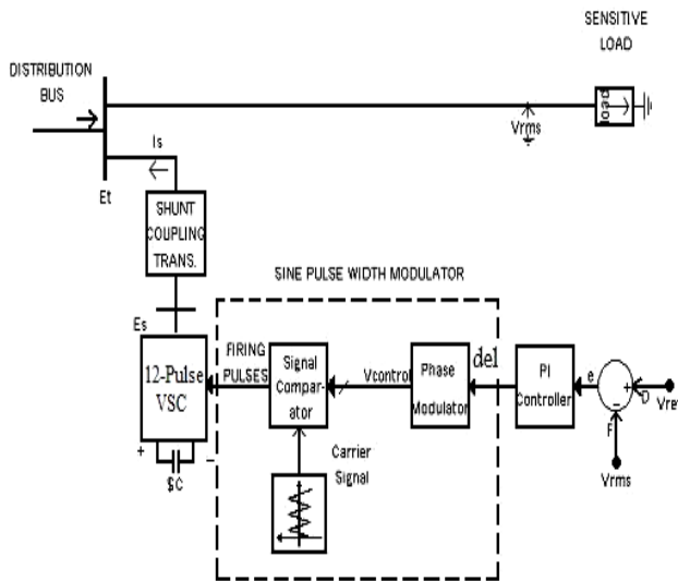
Fig -3 Control scheme designed for the FD-STATCOM
