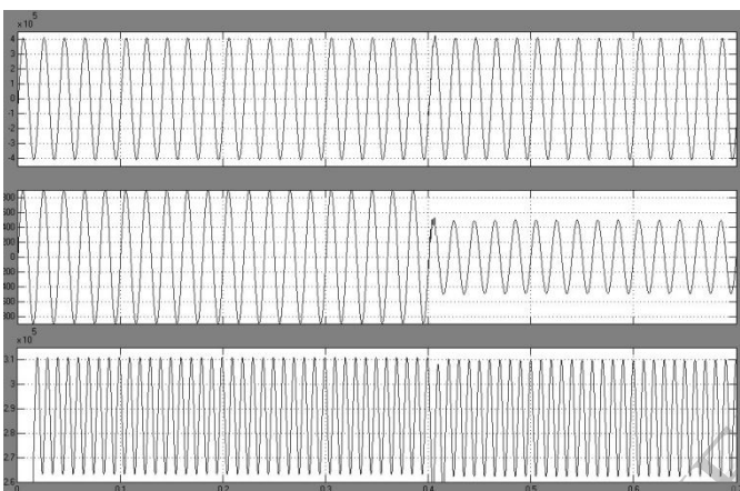
Fig –10 Line Voltage and current when system is subjected to LLLG FAULTS
