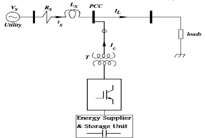
Fig -1 Schematic representation of the FD-STATCOM
