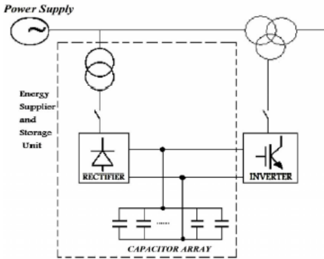
Fig. 4. Structure of SCESS
