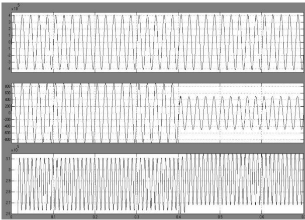
Fig –9 Line Voltage and line current when system is subjected to LG faults
