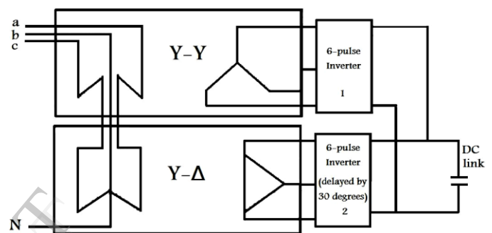
Fig-2 the 12-pulse FD-STATCOM arrangement
