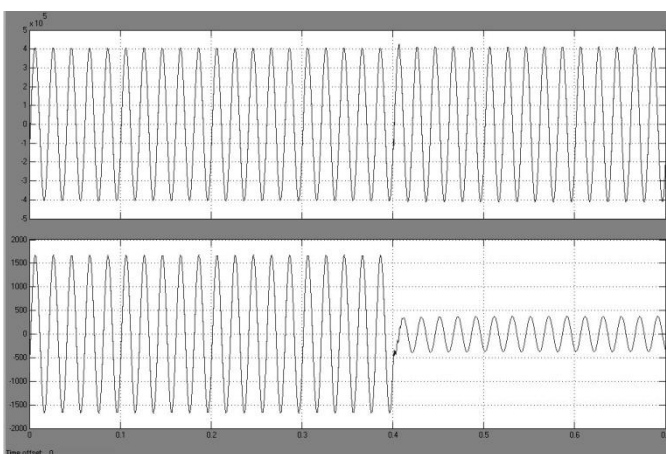
Fig –11 Line voltage and current when system is subjected to LLG FAULT
