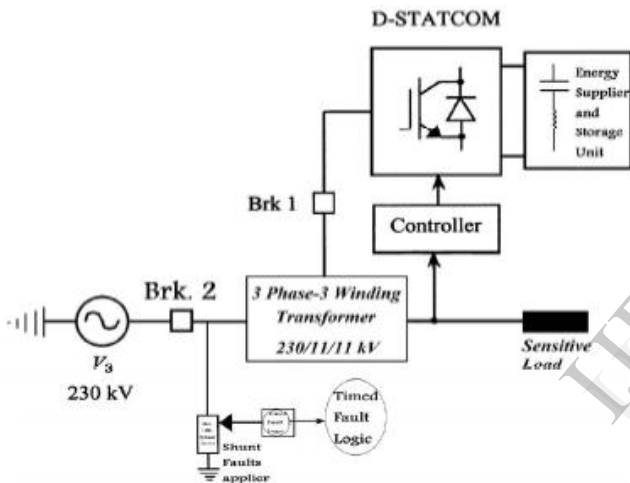
Fig. 5. Distribution system with FD-STATCOM integrated with SCESS and controller
