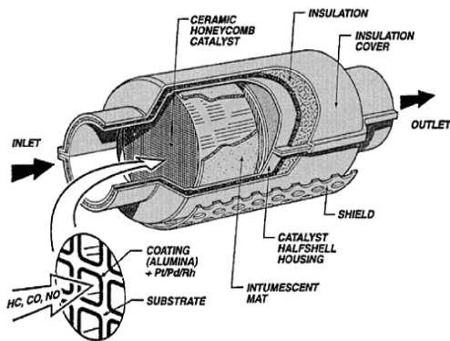
Fig. 1. Anatomy of Catalytic Converter
