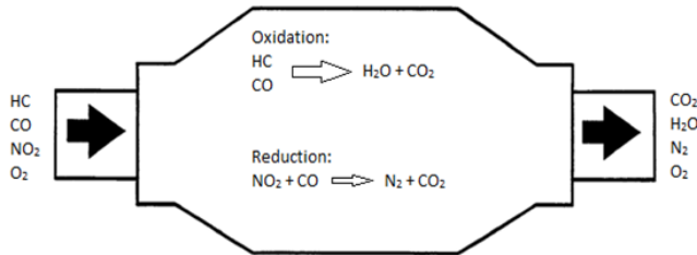
Fig. 2. Working of Catalytic Converter
