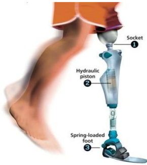
Fig 5: Internal appearance of the artificial leg.
