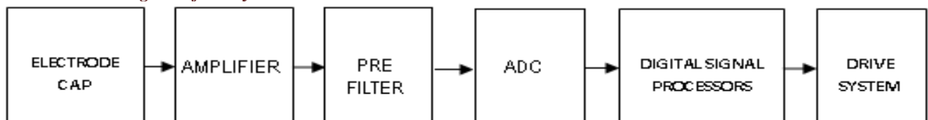
Fig 2: General Block Diagram of the Proposed System
