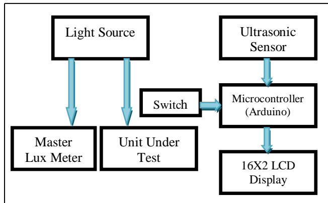
Fig.7. Block Diagram
