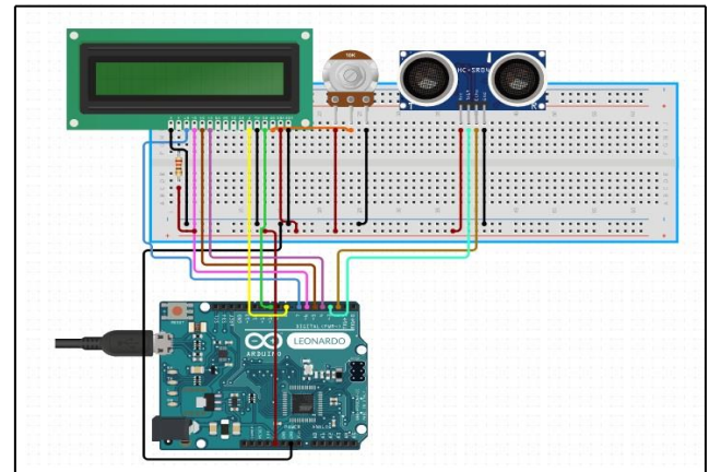
Fig.8. Circuit Diagram
