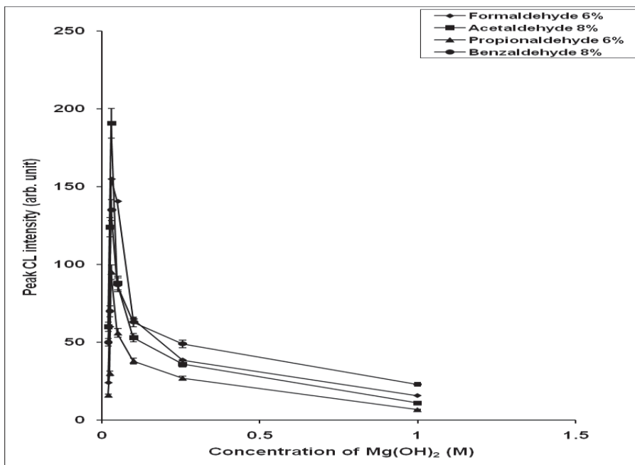
Figure 3: Dependence of peak CL intensity on the concentration of base Mg(OH) 2 under the reaction condition of aldehydes and 20% (w/v) H 2 O 2 at room temperature.
