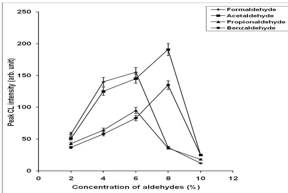
Figure2: Dependence of peak CL intensity on the concentration of aldehydes under the reaction condition of 0.03M Mg(OH) 2 and 20% (w/v) H 2 O 2 at room temperature.
