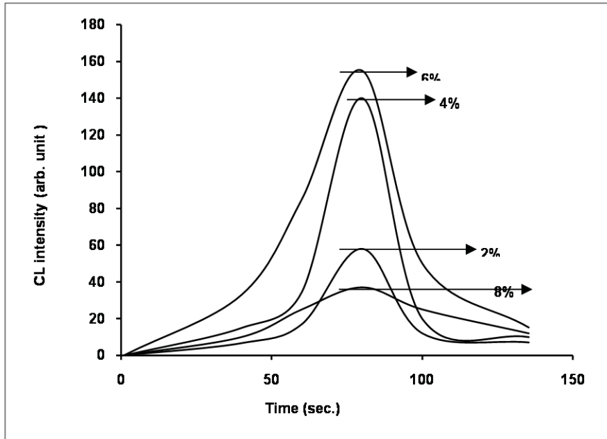
Figure 1: Time dependence of CL intensity on the concentration of formaldehyde (HCHO) under the reaction condition of 0.03M Mg(OH) 2 and 20% (w/v) H 2 O 2 at room temperature.
