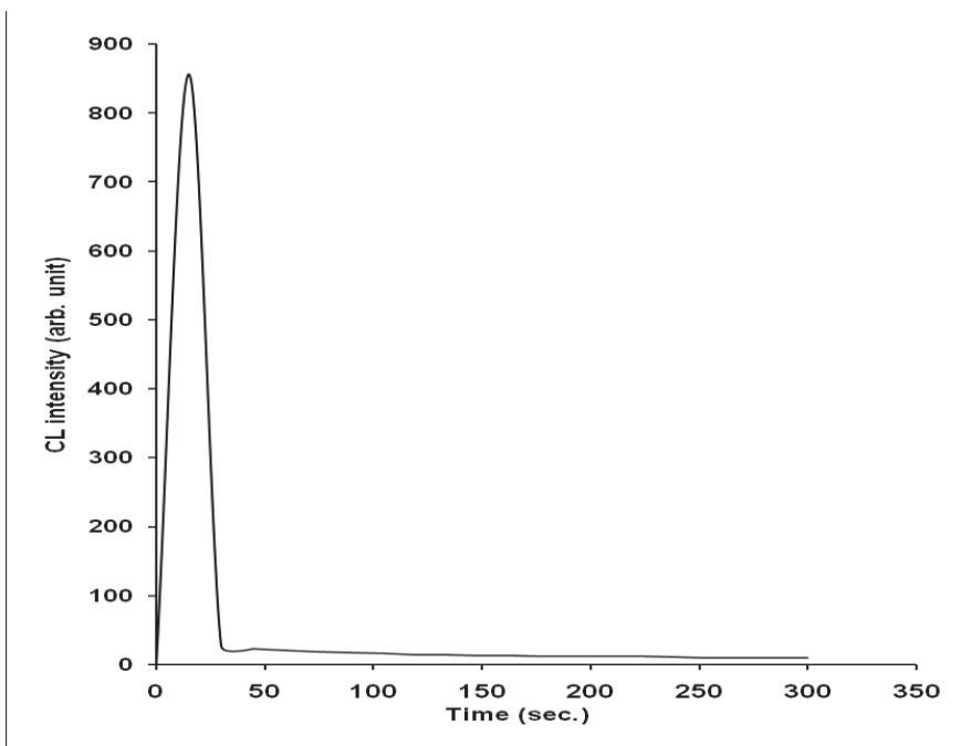
Figure 4: Time dependence of CL intensity of alkaline acetaldehyde (CH 3 CHO) (8%) with hydrogen peroxide in presence of 0.001M luminol at room temperature.
