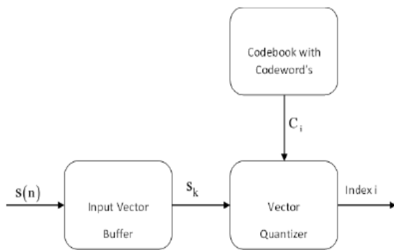
Figure-1. Block diagram of Vector Quantization
