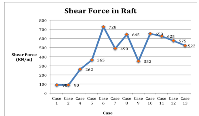
Fig.8 Shear force in raft
