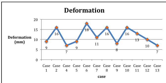
Fig.5 Deformation in each case
