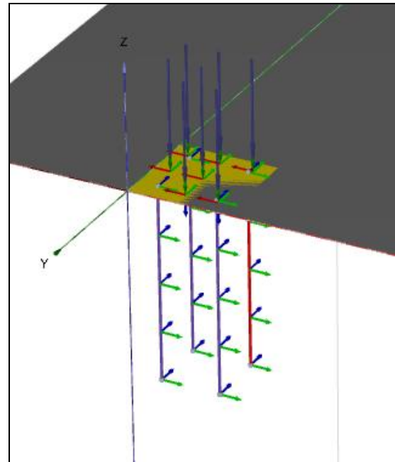
Fig.3 Model of combined pile raft having vertical piles and subjected to vertical load
