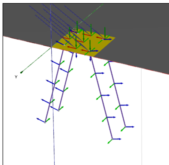
Fig.4 Model of combined pile raft having batter piles and subjected to inclined load
