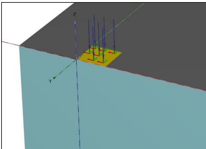
Fig.2 Model of only raft subjected to vertical load
