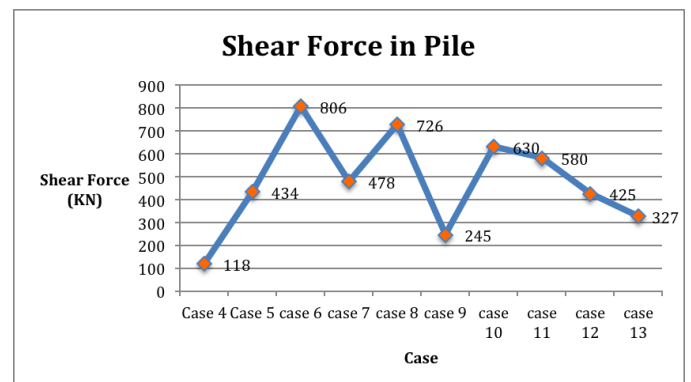
Fig.9 Shear force in Pile
