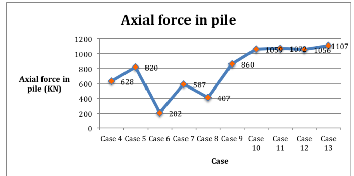
Fig.7 Axial force in pile
