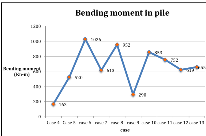
Fig.11 Bending Moment in Pile
