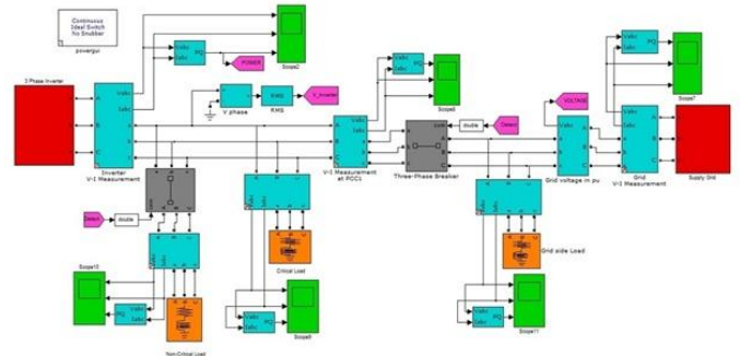
Fig 5: Simulation of current and voltage control block
