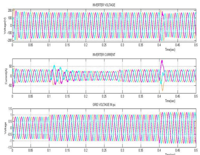
Fig 6: Output waveform of Inverter output voltage and current
