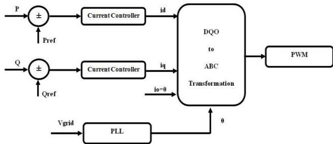
Fig 2: Block diagram representation of Current Control
