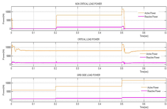
Fig 7: Output waveform of non critical load power, critical load power and grid side load power
