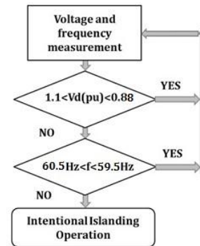
Fig 4: Islanding Detection Algorithm
