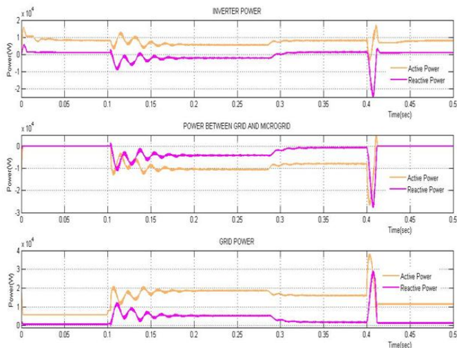
Fig 8: Output waveform of inverter power, power between grid and microgrid and grid power
