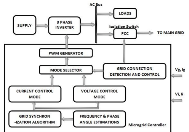
Fig 1: Block diagram representation of Microgrid Controller
