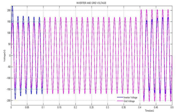
Fig 9: Output waveform of inverter voltage and grid voltage
