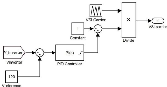
Fig 3: Voltage control during islanded operation
