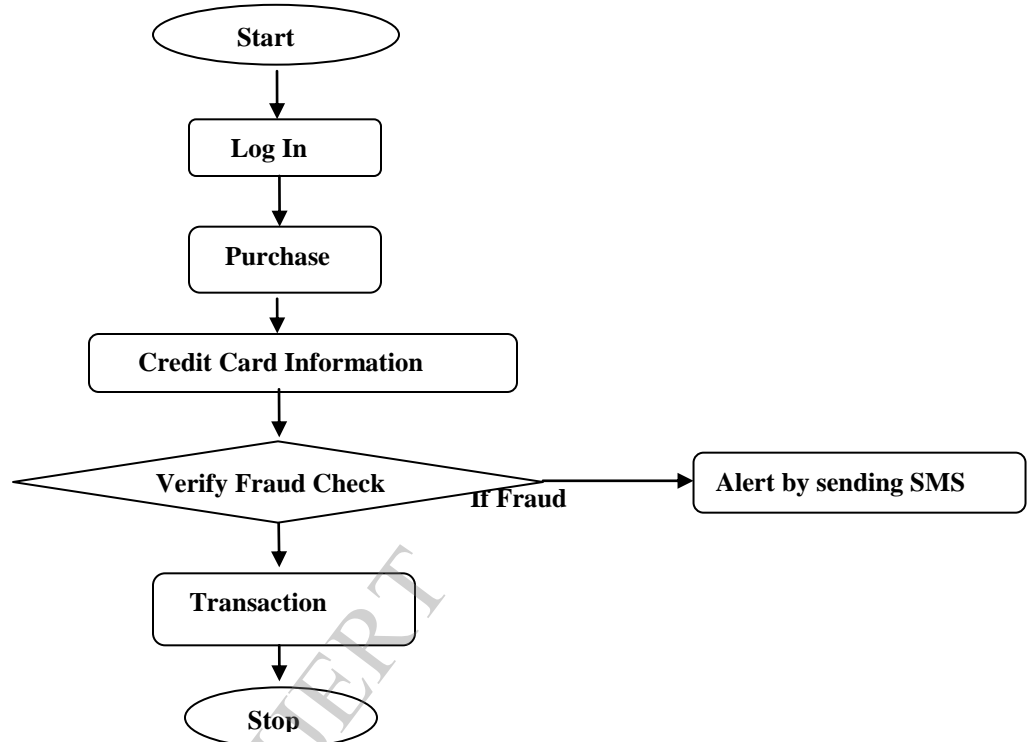
Fig.1: Flowchart of HMM module for credit card fraudulent Detection
