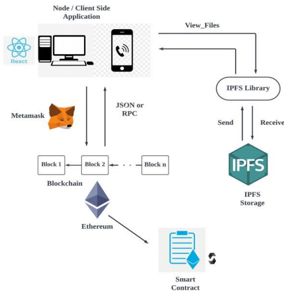
Fig. 3.2 Architecture Diagram of DFS
