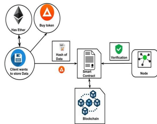
Fig. 3.1 Flow Diagram of DFS
