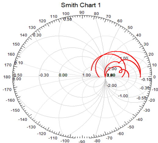
Figure 3(f): Smith chart plot of the proposed antenna
