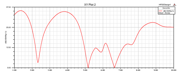
Figure 3(e): VSWR Plot of the proposed antenna
