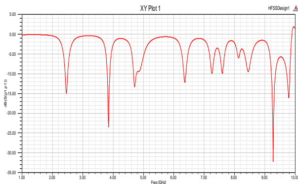
Figure 3(a): plot of return loss VS frequency of the conventional antenna.
