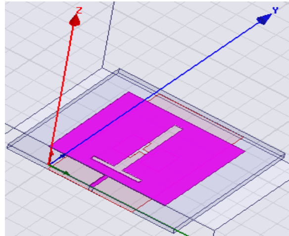
Figure 2(b): Rectangular patch antenna (Front View)
