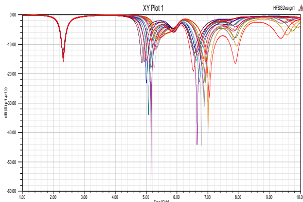
Figure3 (b): return loss VS frequency
