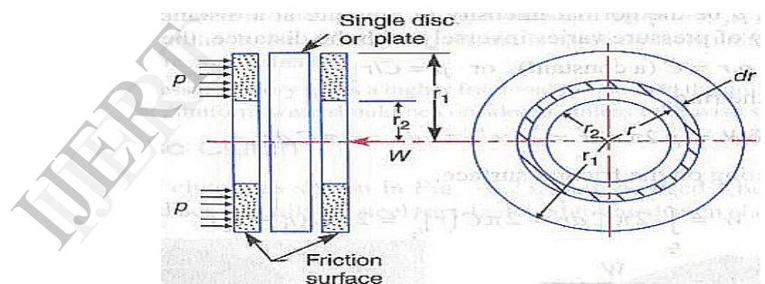
Fig 3. Diagrammatic representation of clutch plate
