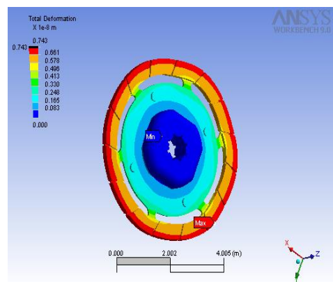
Fig 12.Total Deformation
