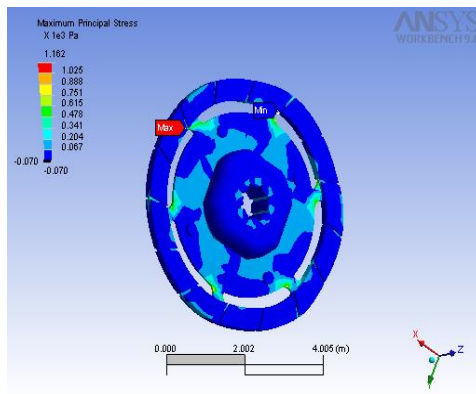
Fig 13.Maximum Principle Stress
