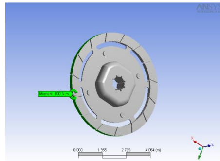
Fig 10. Moment on Plate
