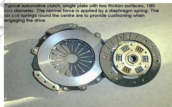
Fig 2. Pressure Plate and clutch Plate in Automotive clutch
