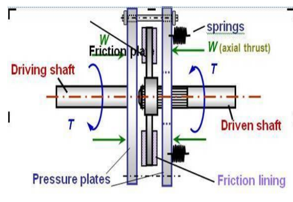
Fig 1. Single Plate Friction Clutch
