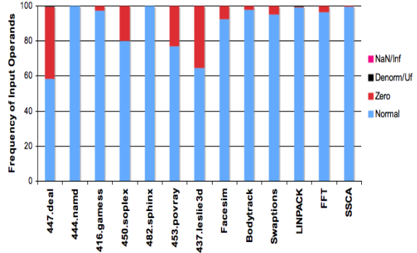
Fig. 9.1: Operand profile of floating-point multiplication instructions
