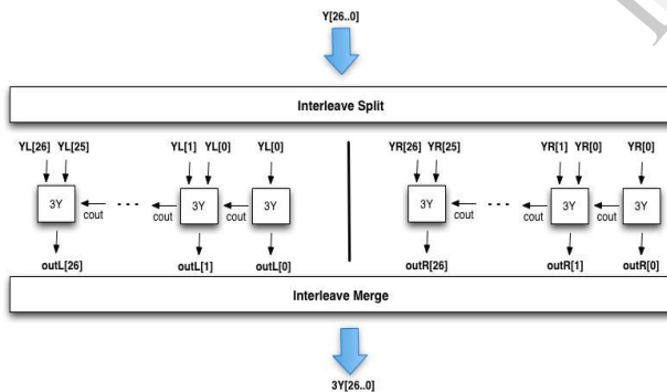
Fig6.2: Radix-4 3Y Adder Longest Carry Length.
