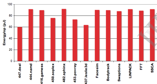
Fig. 10.1: FPM energy per operation across various floating-point applications.
