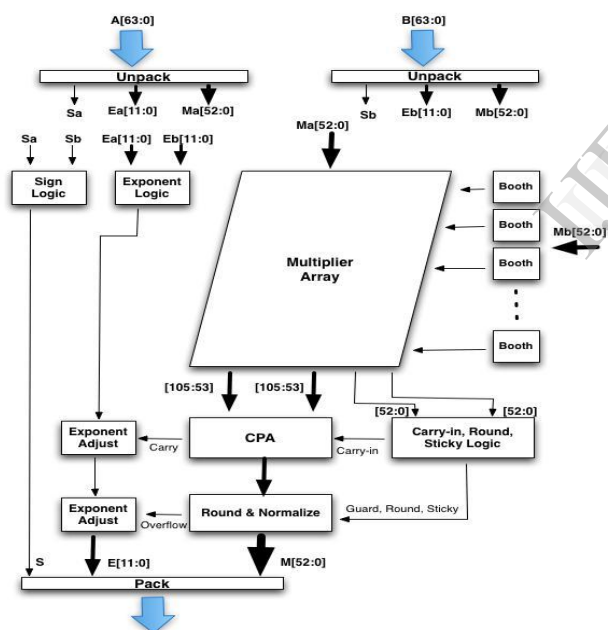
Fig.2.1: Floating-point Multiplier Data path.
