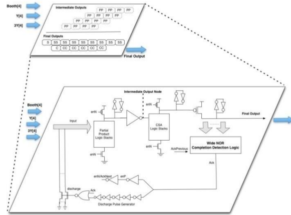
Fig7.2: 8x4 Multiply Logic Block.
