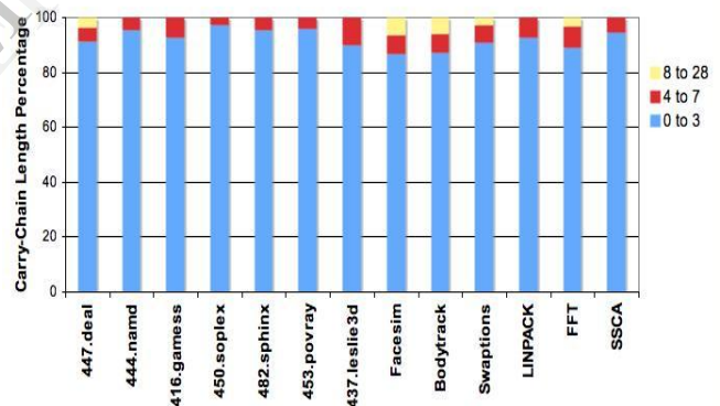
Fig.6.1: Radix-4 3Y Adder Longest Carry Length
