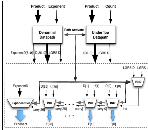
Fig.9.1.Unified rounding hardware for denormal/underflow cases
