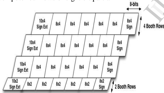
Fig7.1: Radix 8 Multiplier.
