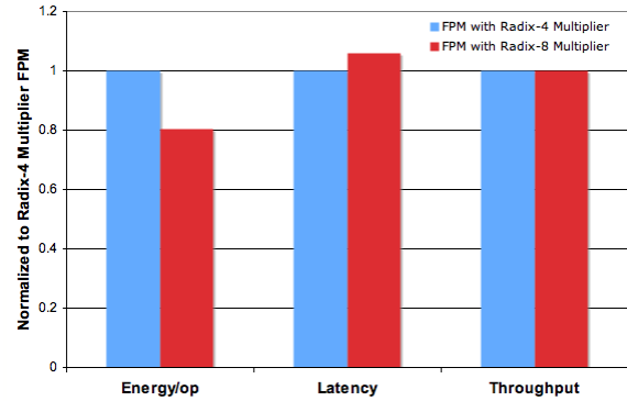
Fig. 7.3. Radix-4 Multiplier vs. Radix-8 Multiplier
