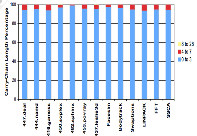
Fig. 10.2 Longest ripple carry Length for Computing CPA Carry input.
