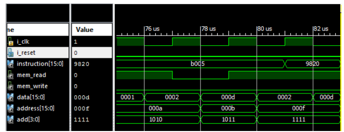
Fig. 20. Waveform of JMP instruction
