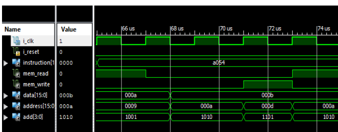
Fig. 19. Waveform of STORE instruction
