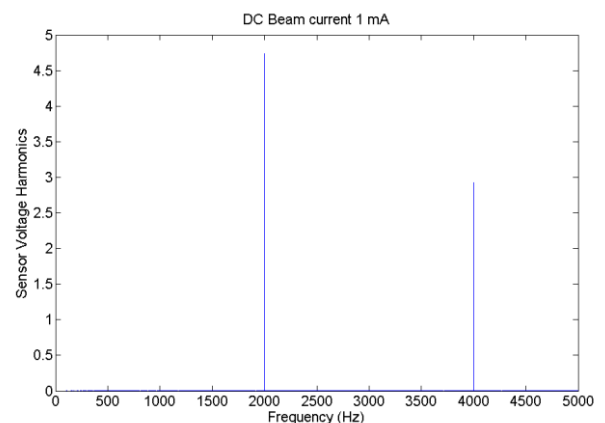
Fig. 5(a): Sensor Voltage harmonics for Vitrovac with H_{\text{sat}}=5\text{A/m} when beam current is 1\text{mA}
