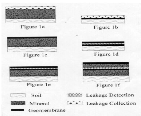
Figure 2.2 Cross section of different liner system (Reddy, 1999)
