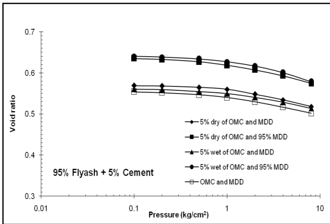
Figure 4.7 e - \log p plots of 95% fly ash + 5% cement with different compaction conditions
