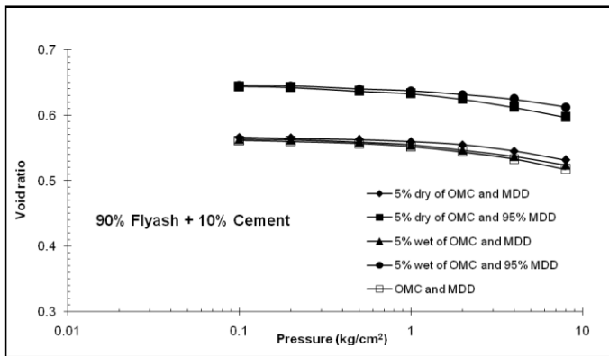
Figure 4.8 e - \log p plots of 90% fly ash + 10% cement with different compaction conditions
