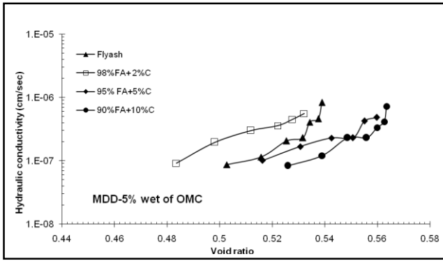
Figure 4.12 e - \log k plots of different mix compacted with 5% Wet of OMC and MDD
