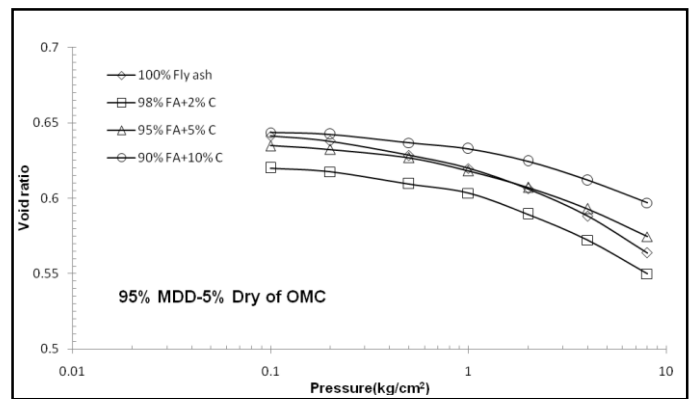
Figure 4.16 e - \log p plots of different mix compacted with 5% Dry of OMC and 95% MDD
