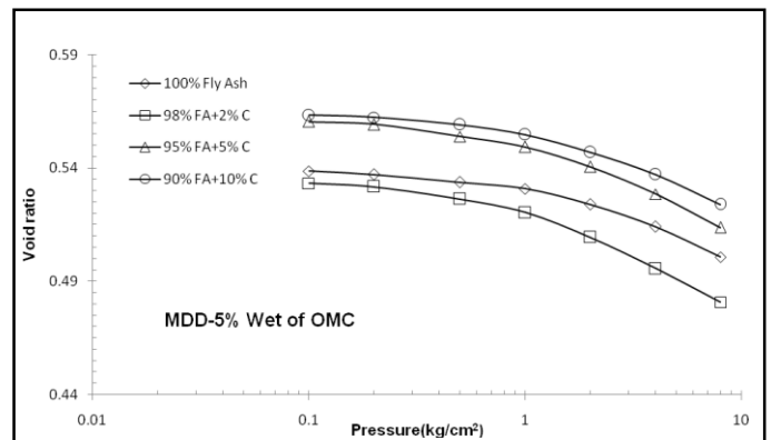
Figure 4.17 e - \log p plots of different mix compacted with 5% Wet of OMC and MDD
