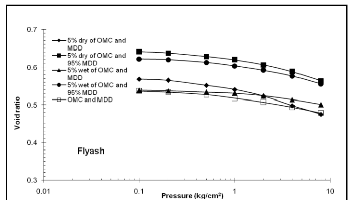
Figure 4.5 e - \log p plots of fly ash with different compaction conditions
