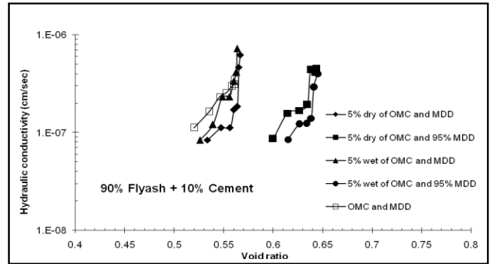
Figure 4.4 e - \log k plots of 90% fly ash + 10% cement with different compaction conditions
