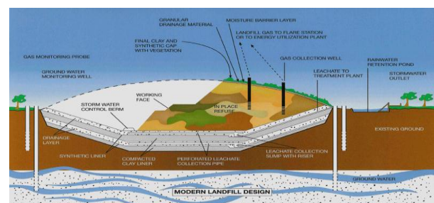
Figure 2.1: Cross section of landfill components (Reference)
