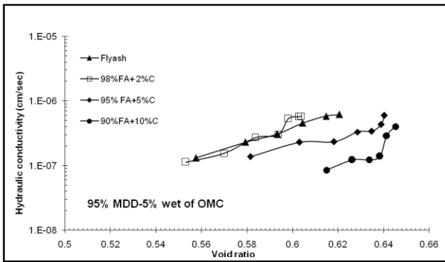
Figure 4.13 e - \log k plots of different mix compacted with 5% Wet of OMC and 95% MDD
