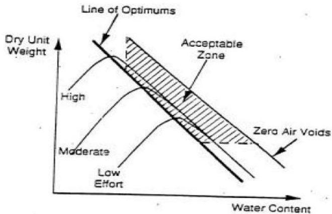
Figure 2.6 Acceptable zone of dry density and moisture content with compactive efforts (Cawley 1999)
