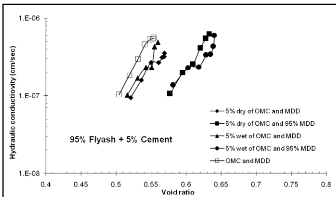
Figure 4.3 e - \log k plots of 95% fly ash + 5% cement with different compaction conditions
