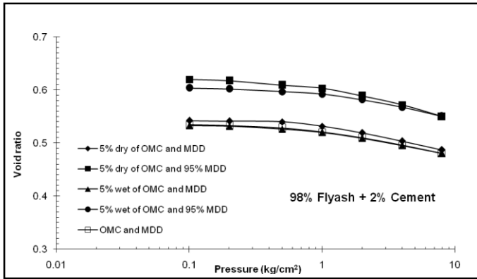
Figure 4.6 e - \log p plots of 98% fly ash + 2% cement with different compaction conditions
