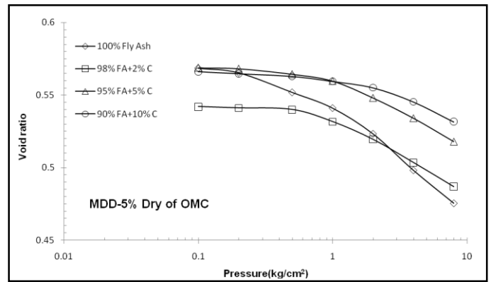
Figure 4.15 e - \log p plots of different mix compacted with 5% Dry of OMC and MDD
