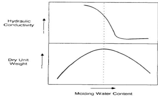
Figure 2.4 Variation of hydraulic conductivity, dry density and molding water content
