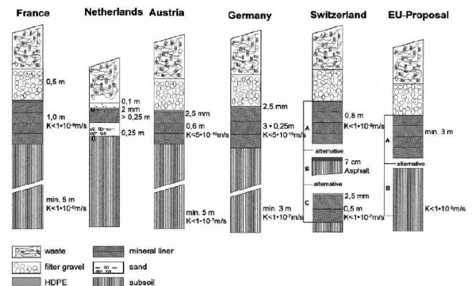
Figure 2.3 National regulations of landfill liners (Dietrich, 2002)
