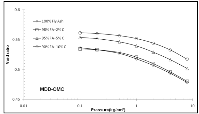
Figure 4.14 e - \log p plots of different mix compacted with OMC and MDD
