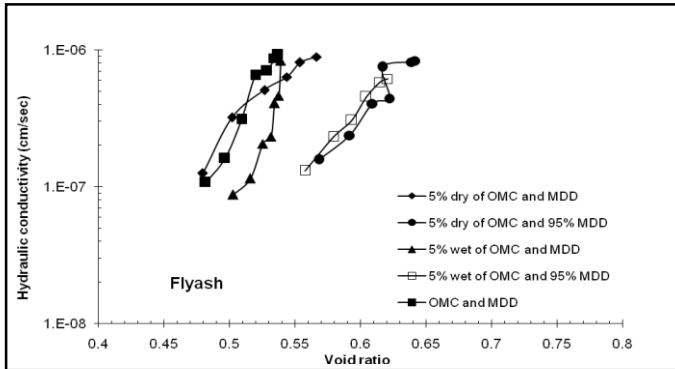
Figure 4.1 e - \log k plots of fly ash with different compaction conditions
