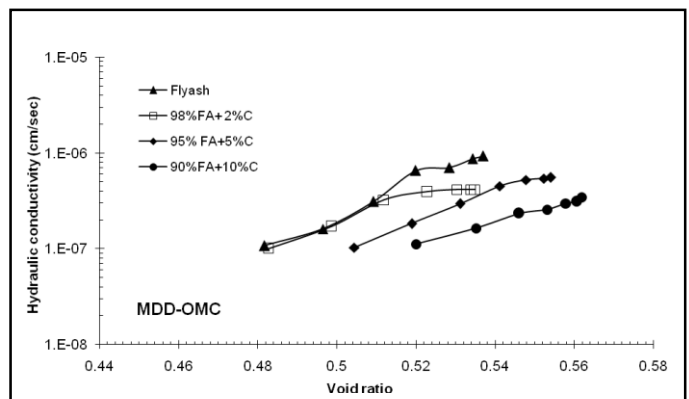
Figure 4.9 e - \log k plots of different mix compacted with OMC and MDD
