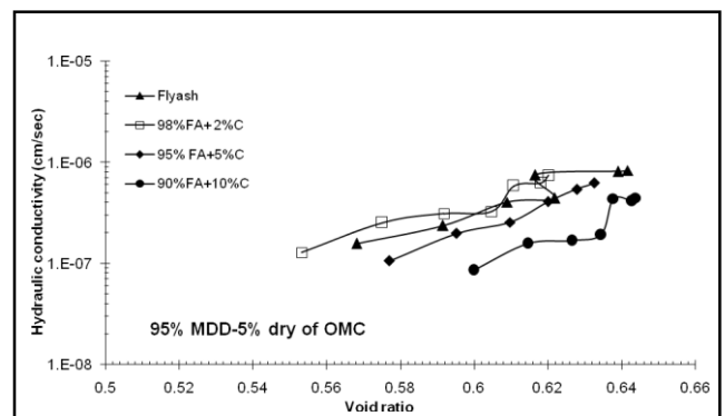
Figure 4.11 e - \log k plots of different mix compacted with 5% Dry of OMC and 95% MDD
