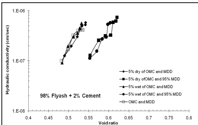
Figure 4.2 e - \log k plots of 98% fly ash + 2% cement with different compaction conditions
