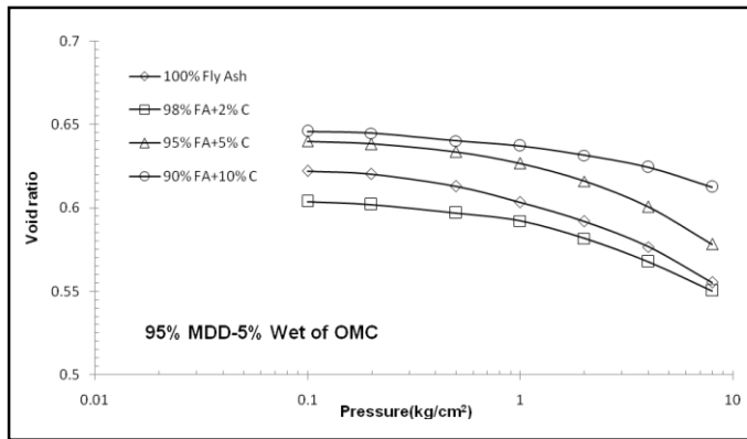
Figure 4.18 e – log p plots of different mix compacted with 5% Wet of OMC and 95% MDD
