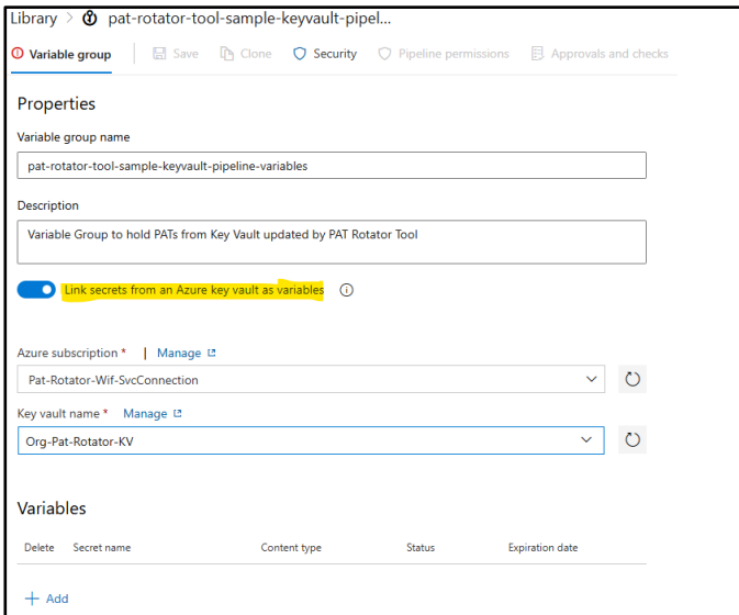
Fig. 1. ADO Pipelines Library - Variable Groups
