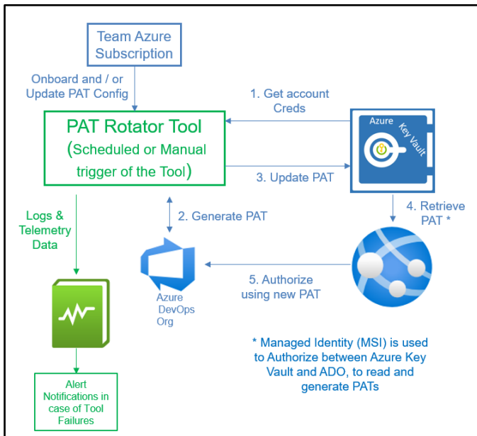
Fig. 2. PAT Rotator Tool Workflow
