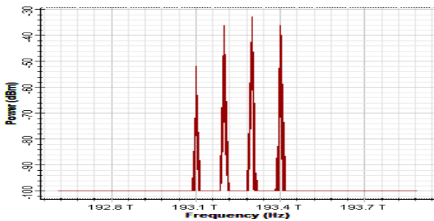
Figure 13: Optical Spectrum which shows that there is no fiber cut in the PON system
