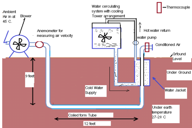
Fig.2.1 Experimental Set up of EAPHE
