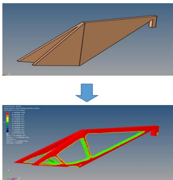
Fig. 19. Initial to optimized design
