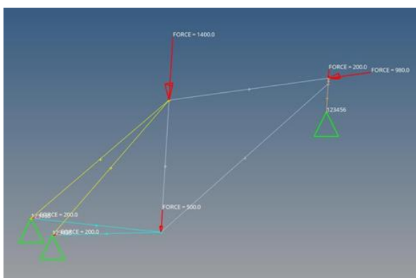
Fig. 1. Loading and boundary conditions
