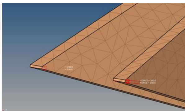
Fig. 7. Loading conditions
