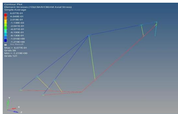
Fig. 21. Element stresses of optimized model
