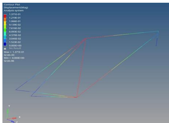
Fig. 14. Total displacement of bamboo bike frame
