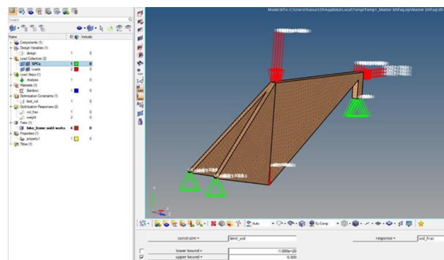
Fig. 12. Constraint implementation for topology optimization
