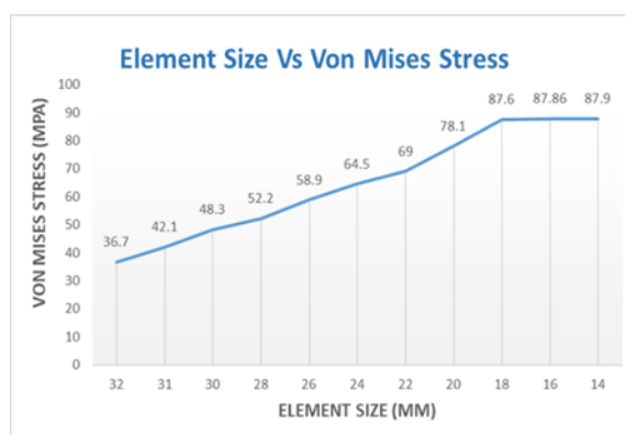
Fig. 2. Graph between element size and von mises stress
