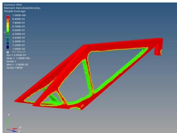
Fig. 18. Optimized design of bamboo bike frame
