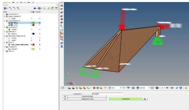
Fig. 11. Setting responses for topology optimization
