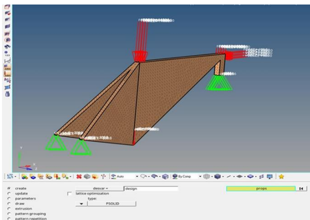
Fig. 10. Establish design parameters
