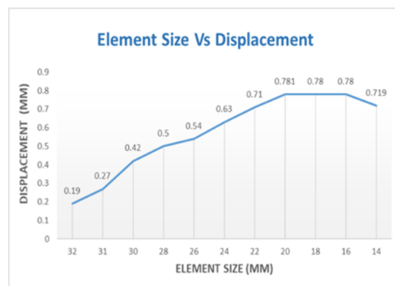
Fig. 3. Graph between element size and displacement
