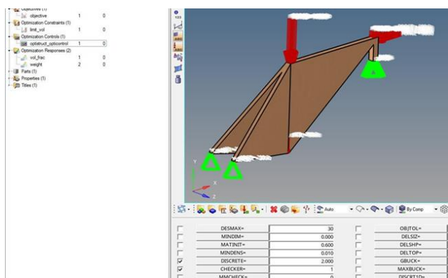
Fig. 13. Setting opticontrol panel for optimization
