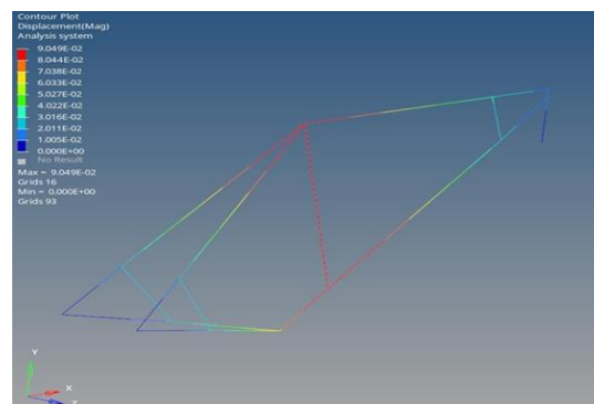
Fig. 22. Total displacement of optimized model
