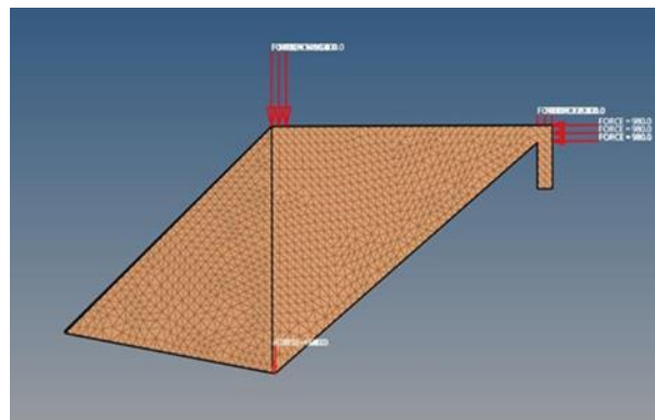
Fig. 6. Loading conditions
