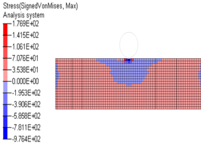
Fig.4 Stress contour at shot speed 15 m/s
