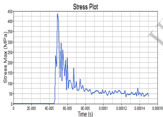
Fig.9 Stress plot at shot speed 20m/s
