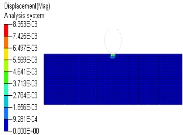
Fig.6 Displacement contour at shot speed 15m/s
