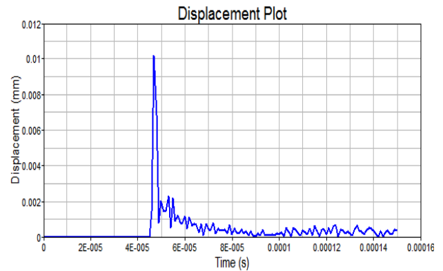
Fig.10 Displacement plot at shot speed 20m/s
