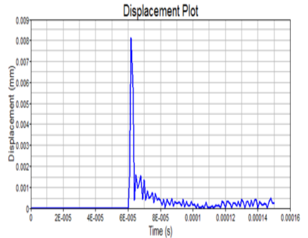
Fig.7 Displacement plot at shot speed 15m/s
