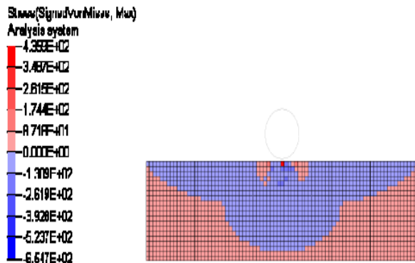
Fig.8 Stress contour at shot speed 20 m/s
