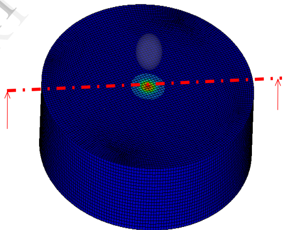
Fig.3 Shot impact zone.
