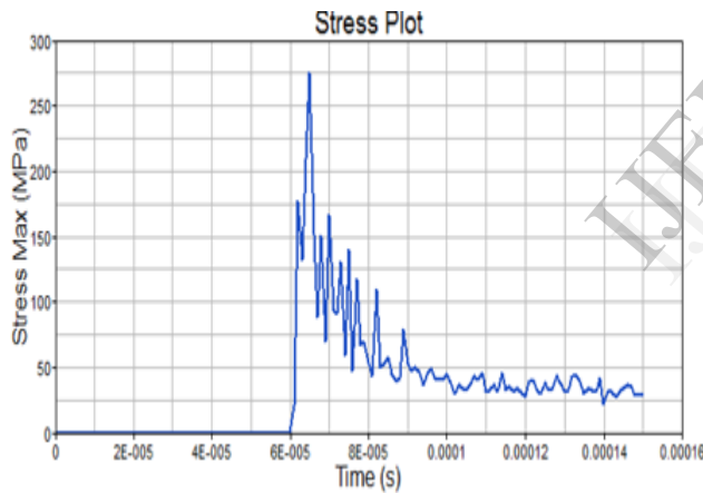
Fig.5 Stress plot at shot speed 15m/s
