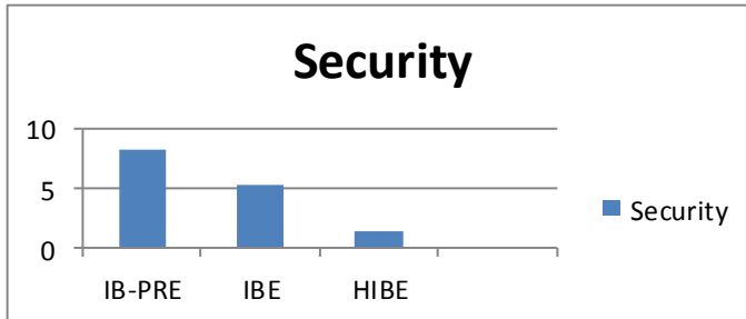
Fig 2. Security Analysis
