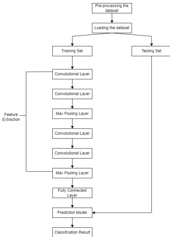
Fig. 4. Flowchart of CNN Model 1 for Bengali characters
