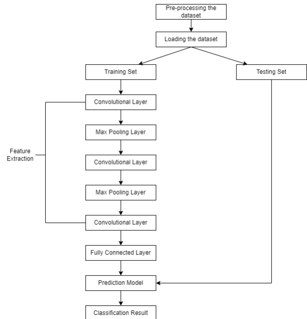
Fig. 5. Flowchart of CNN Model 2 for Bengali characters
