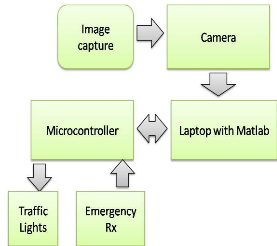
Figure 1 Block Diagram of Image processing based Traffic Control System
