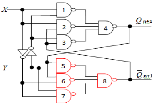
Figure 4.1(a): Logic Circuit of XY-FF No Rest at 100% (NAND Gate Configuration)
