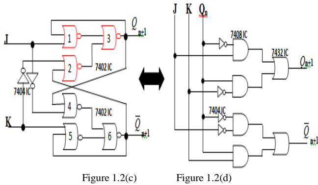
Figure 1.2(c): NOR gates JK-FF based on K-map Figure 1.2(d): NOT, AND & OR gates JK-FF based on characteristic equations
