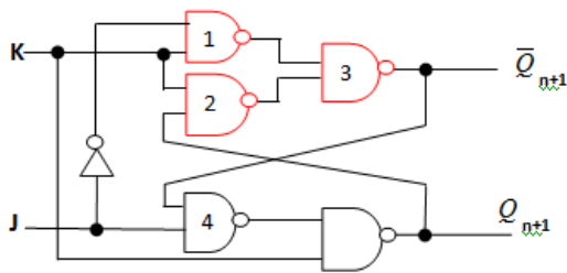
Figure 3.1(a): Logic Circuit of JK-FF Extension – 1 at 87.5% (NAND Gate Configuration)
