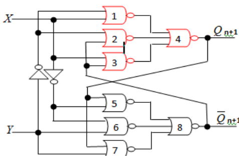
Figure 4.1(b): Logic Circuit of XY-FF No Rest at 100% (NOR Gate Configuration)
