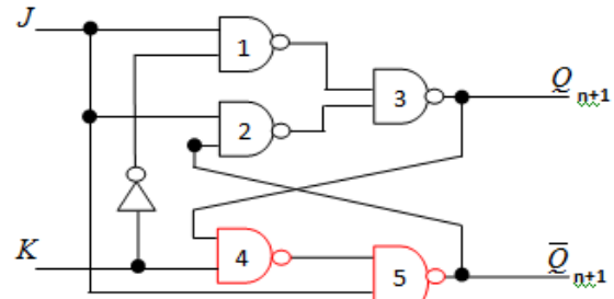
Figure 2.1(a): Logic Circuit of JK-FF Extension – 0 at 87.5% (NAND Gate Configuration)
