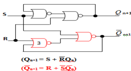
Fig. 1.2(a): SR NOR gates Flip Flop Equation Omotosho & Ogunlere (2013)
