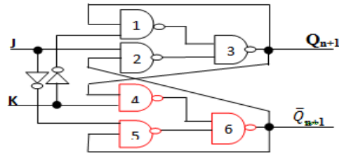
Figure 1.2 (a): Logic Circuit of Conventional JK-Flip Flop - 75% (NAND Gate Configuration.)
