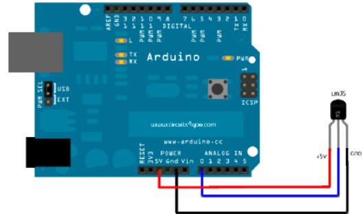
Figure 6: Connection Circuit with LM35 Sensor
