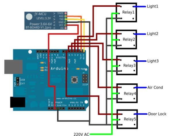
Figure 3: Hardware architecture and implementation
