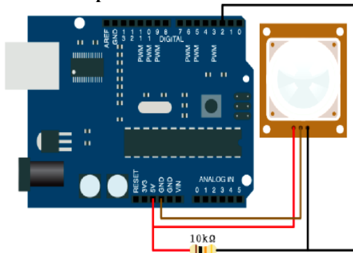
Figure 5: Connection Circuit with PIR Sensor
