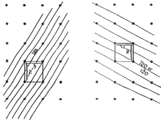
Fig. 2: Two – dimensional representation of a lattice, showing conditions for reflection and the method of defining planes.
