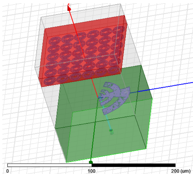
Fig.4.2 The 3-D view of proposed antenna
