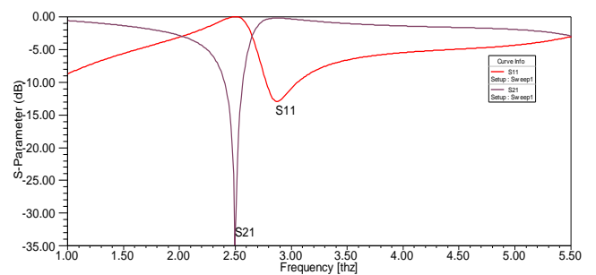
Fig.3.3 The simulated S_{11} and S_{21} of the CSRR with respect to frequency
