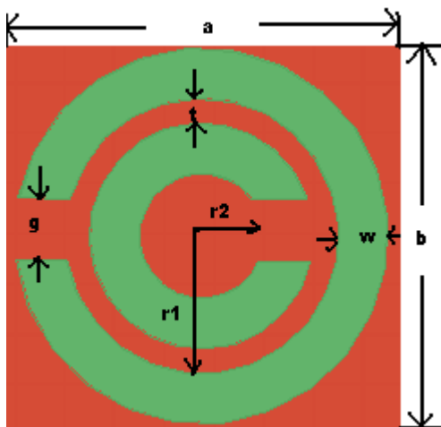
Fig.3.1 A top view of the CSRR metamaterial unit cell
