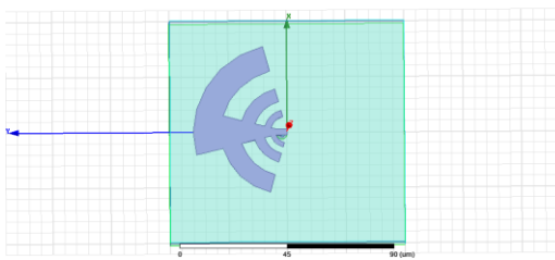
Fig.4.1 The top view of log-periodic terahertz antenna without metamaterial.
