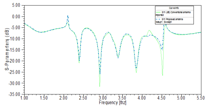
Fig.4.3 The simulated S_{11} parameters of conventional antenna (continuous line) and proposed antenna (dashed line)
