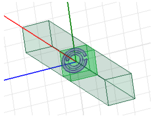
Fig. 3.2 The simulation setup in HFSS for unit cell
