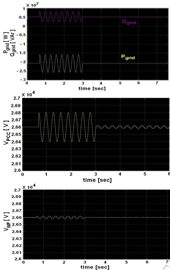
Figure 11. (a) Active and Reactive power demand at power grid side. (b) PCC Voltage. (c) WF terminal voltages
