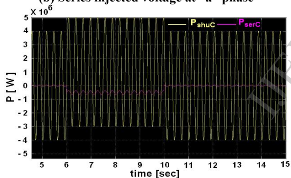
Figure 14. Shunt & Series converter active power
