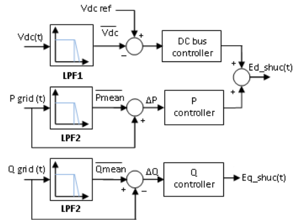
Figure 6. Shunt compensator controller
