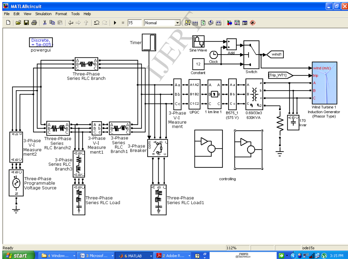
Figure 8. Model of power system scheme illustrated in Figure 1
