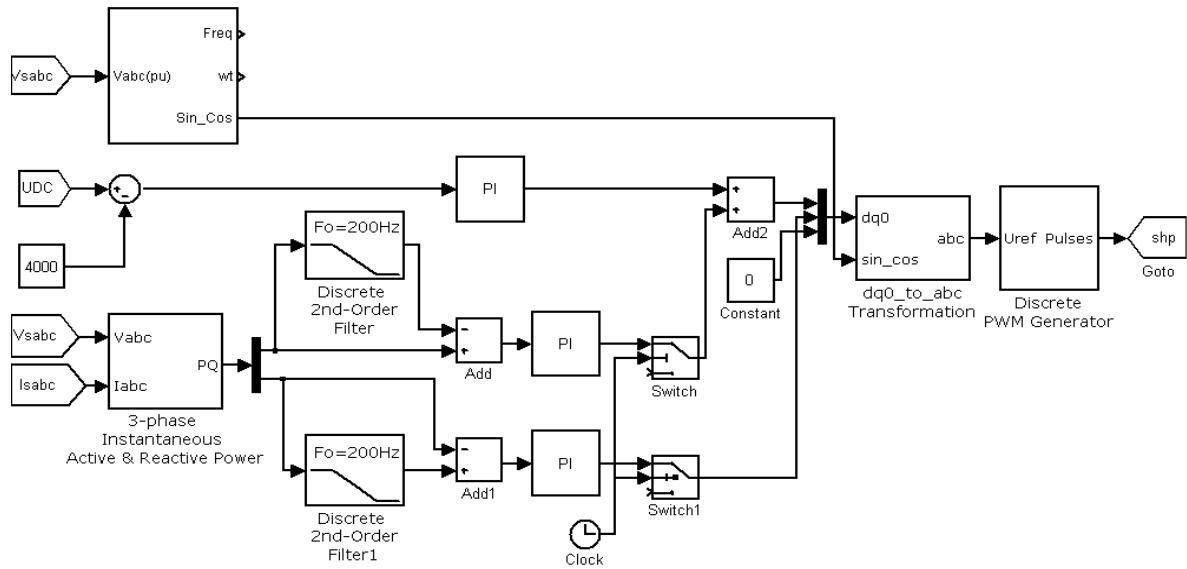
Figure 9. Shunt controller circuit
