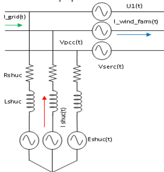
Figure 4. Power stage compensator model. AC side
