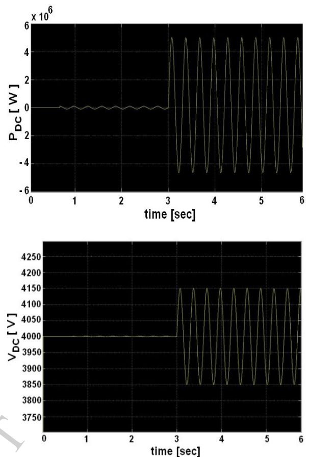
Figure 12. (a) Power of the capacitor in the DC-Bus. (b) Voltage of the capacitor in the DC-Bus.
