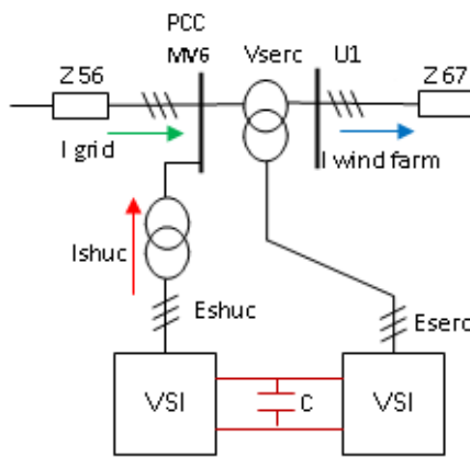
Figure 2. Block diagram of UPQC
