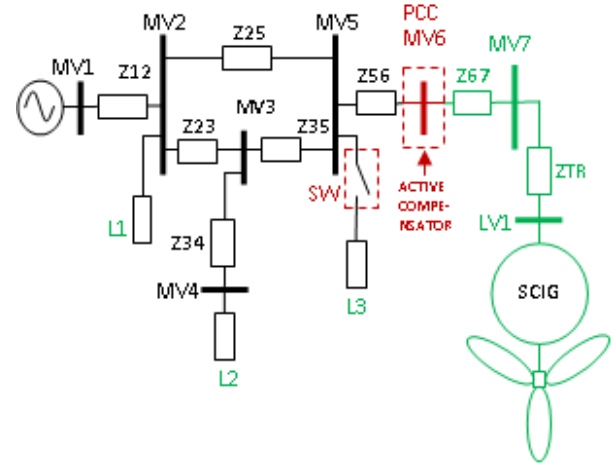
Figure 1. Study case Power system
