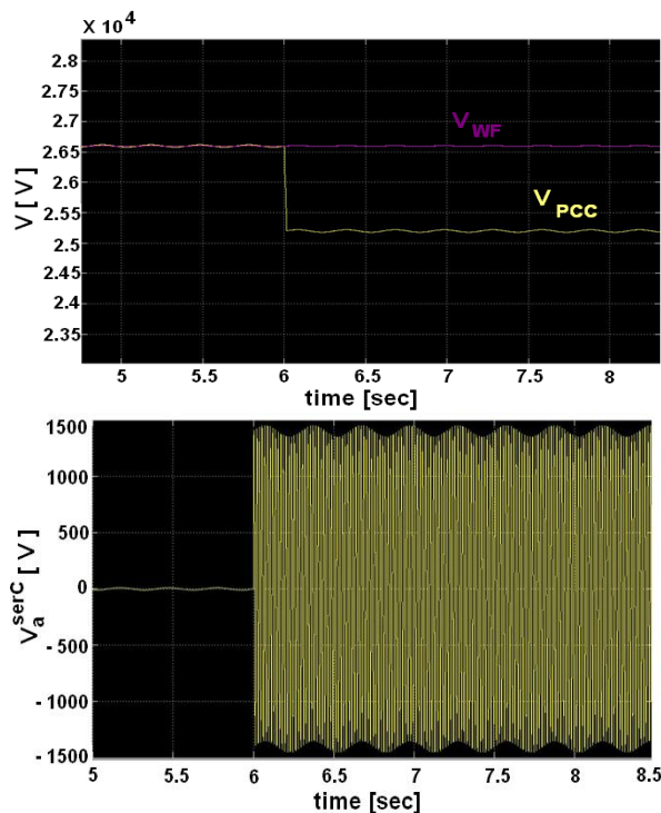
Figure 13. (a) Voltage at WF, at PCC. (b) Series injected voltage at "a" phase
