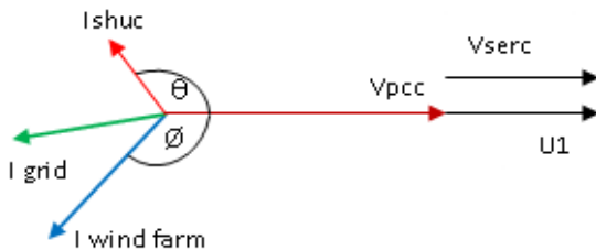
Figure 3. Phasor diagram of UPQC
