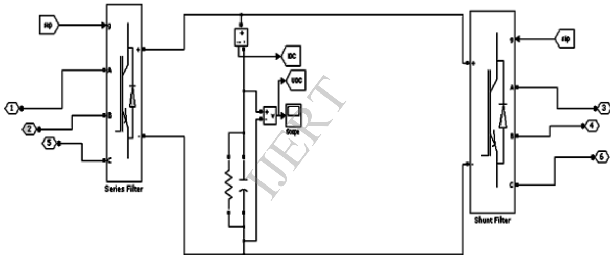
Figure 10. UPQC Circuit
