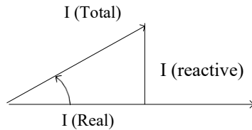
Fig.3 The concept of leading power factor POWER FACTOR IMPROVEMENT
