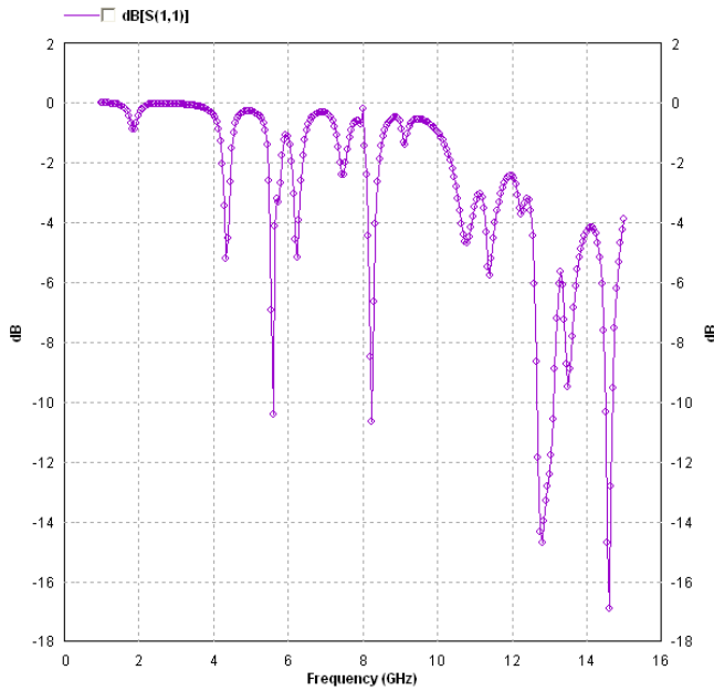
Figure 4 Simulated Return Loss (S11) Of Rectangular Fractal Antenna
