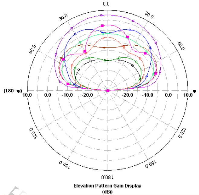
Figure 6 Elevation Pattern Gains Display (dbi)
