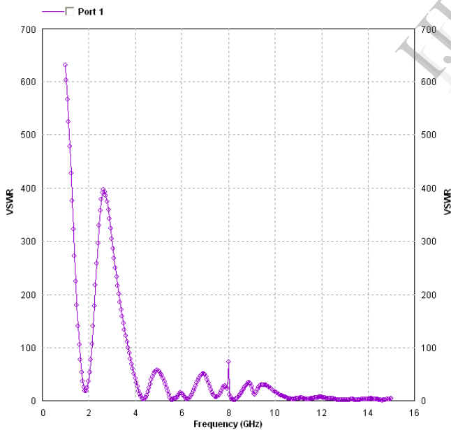
Figure 5 VSWR –Frequency Characteristic
