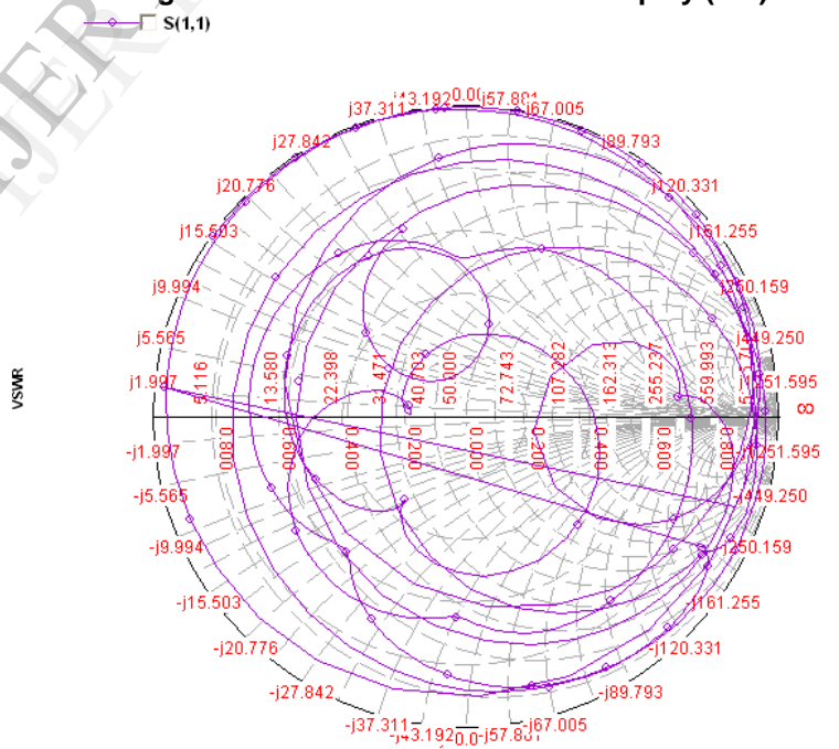
Figure 7 Smith Chart
