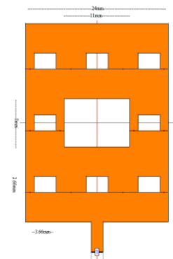
Figure 3 Proposed Antenna And Its Geometry Of Second Iteration
