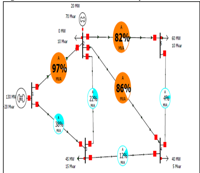
Fig 4 Shows the modified IEEE 5- bus system with out TCSC
