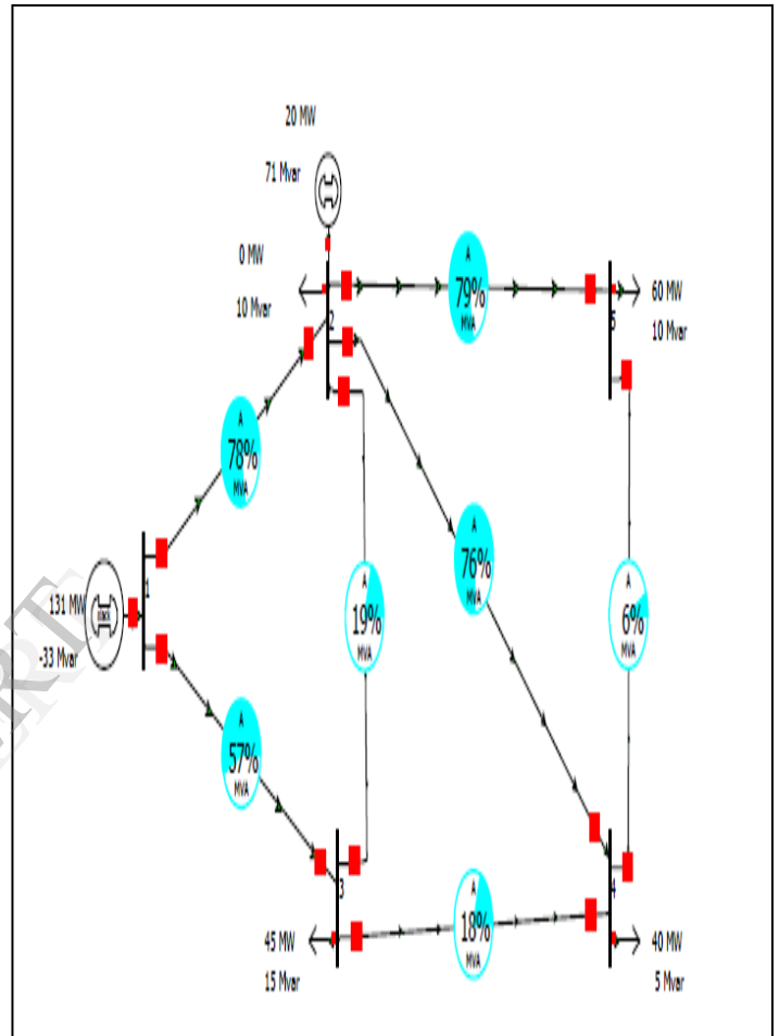
Fig 6 Shows the modified IEEE 5- bus system With TCSC (Overloading mitigation by TCSC)
