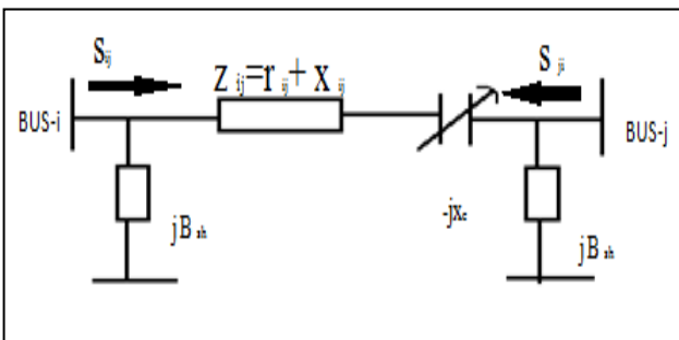
Fig 2. Injection Model of TCSC
