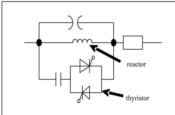
Fig 1. Equivalent circuit of TCSC
