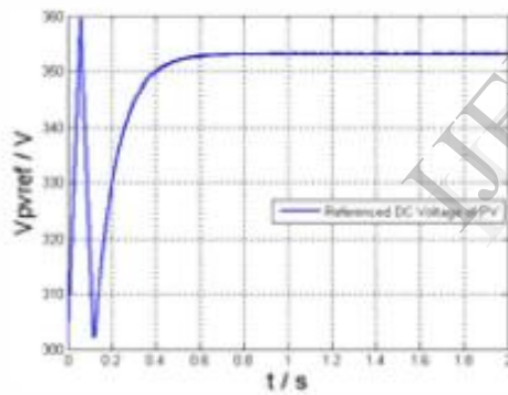
(a) DC reference voltage
