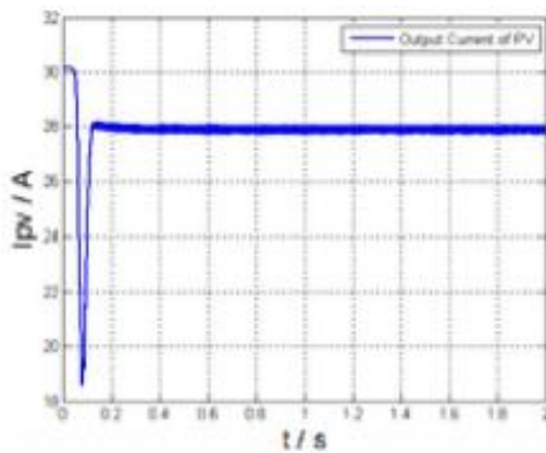
(c) Output current of PV array
