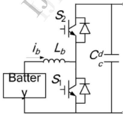
Figure 8. The bi-directional DC/DC converter.
