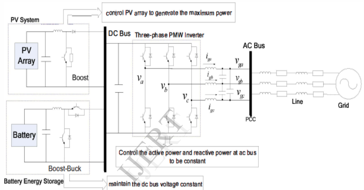
Figure 6, Configuration of the grid-connected hybrid PV /Battery generation system.
