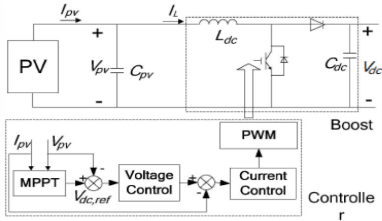
Figure 7, Boost circuit and its control
