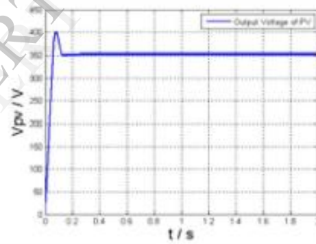
(b) Output voltage of PV array
