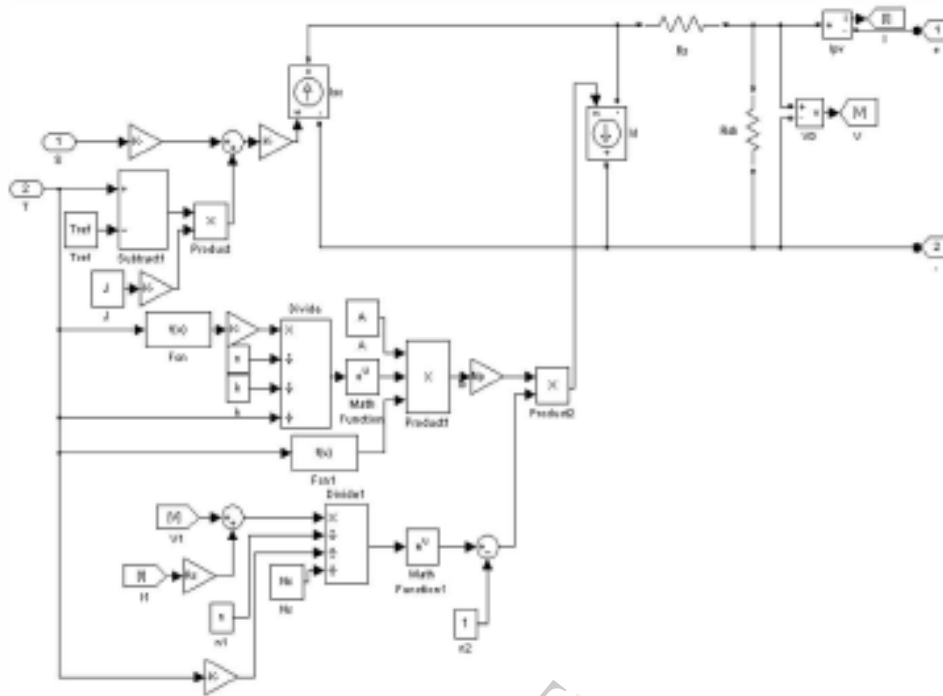
Figure 2, The model of PV array in MATLAB/Simulink With different temperatures and solar radiations, output characteristics of PV array are simulated as figure 3 and figure 4.
