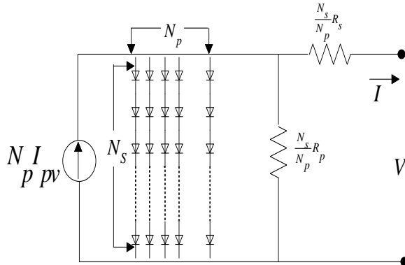
Fig 1. General Equivalent circuits Model of generalized PV array The terminal equation for the current and voltage of the array becomes as follows
