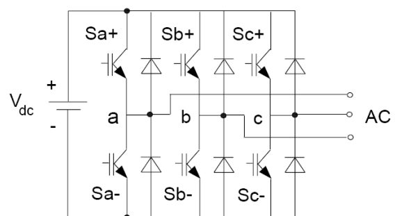
Fig 7. Grid connected IGBT inverter system
