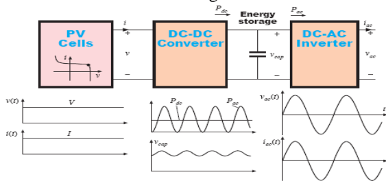
Fig 8. Behavior of V & I from PV cell to inverter
