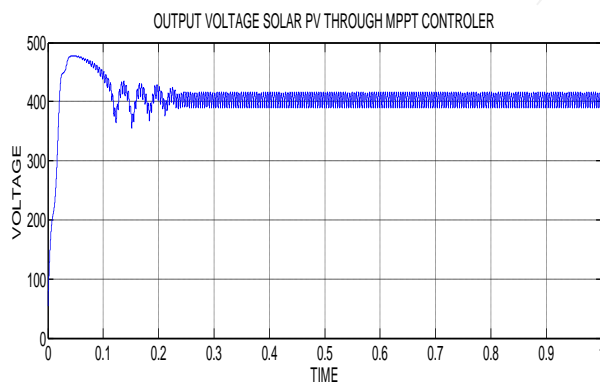
Fig 19 .output voltage of solar pv system
