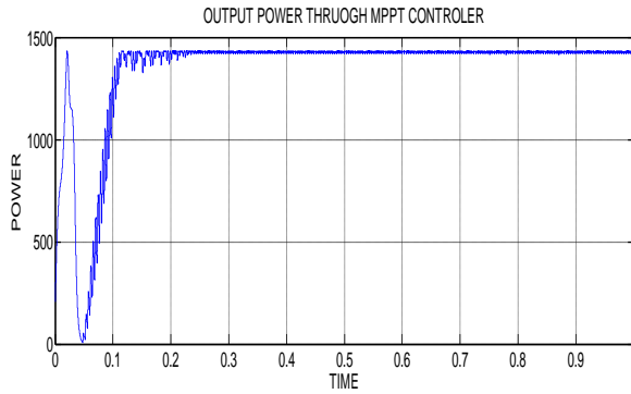
Fig 10. MPPT controller output of solar PV system
