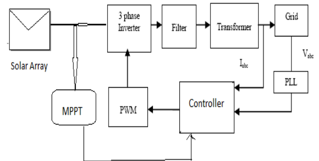
Fig 9. Over all block diagram of system
