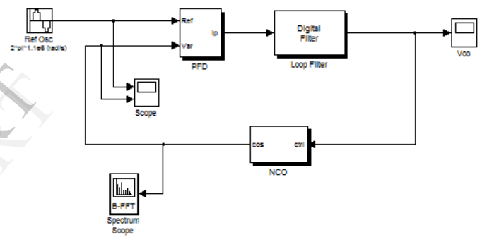
Fig 6. Simulink model of PLL
