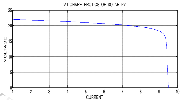
Fig 4. V-I characteristics of solar PV
