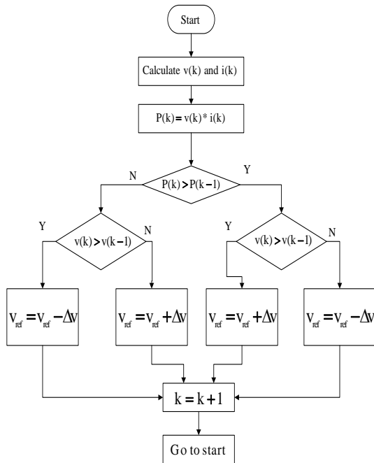
Fig 5. P & O observation technique
