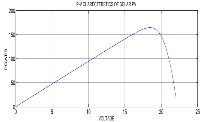
Fig 3. P-V characteristics of solar PV
